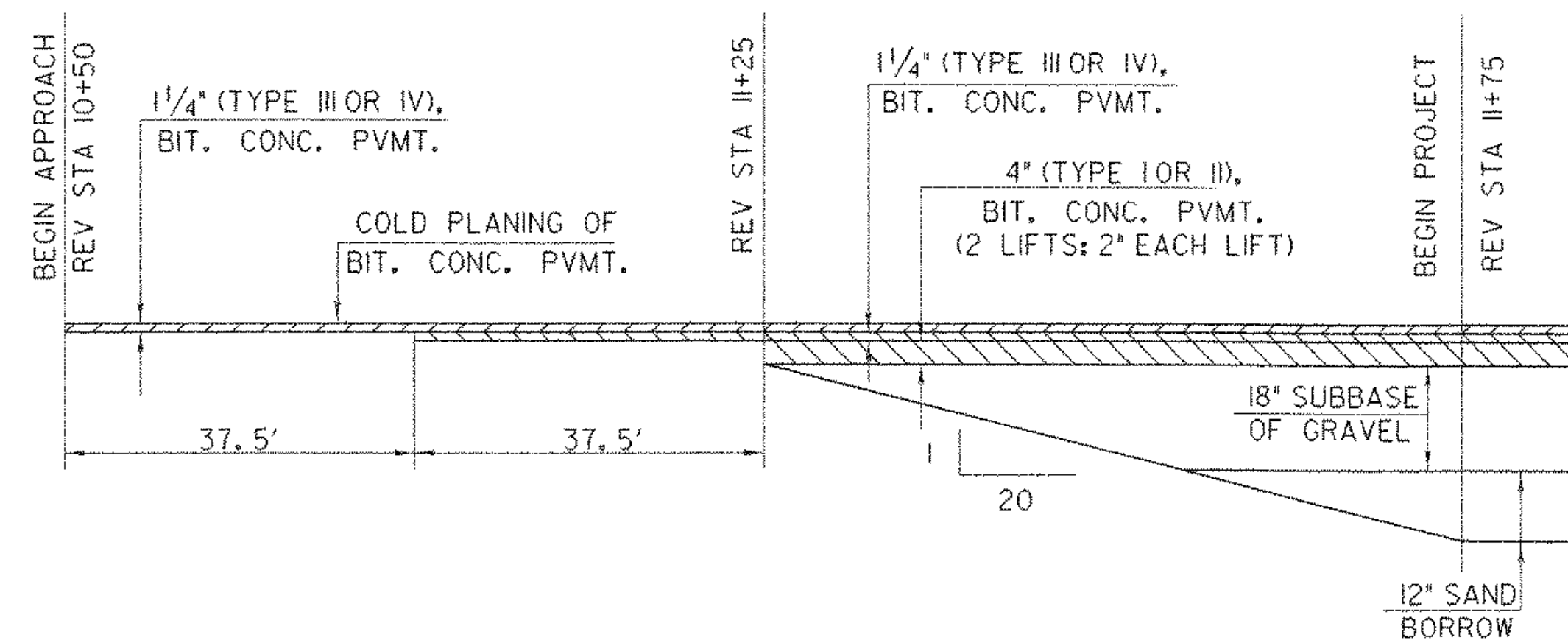
SUBBASE TRANSITION NTS
