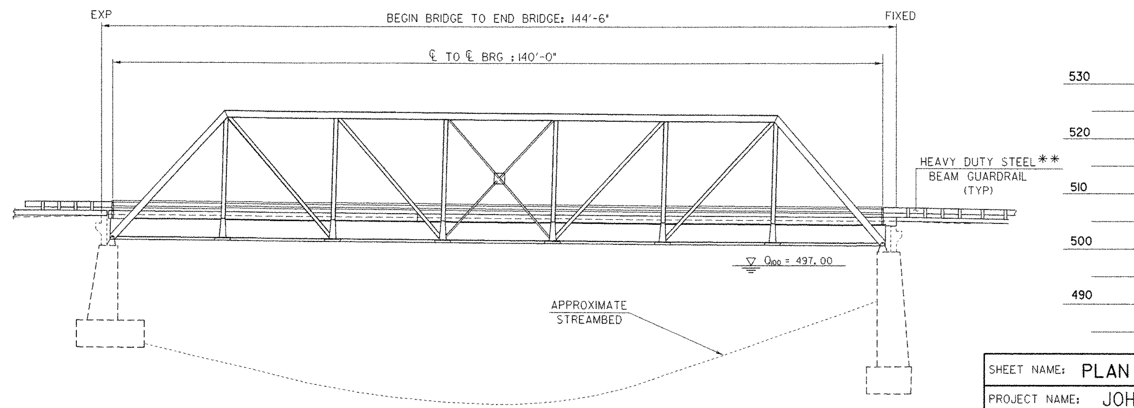
ELEVATION @ UPSTREAM FASCIA OF TRUSS SCALE 1" = 10'-0"
