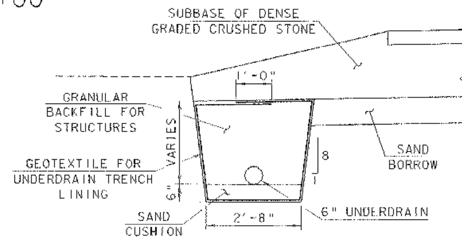
UNDERDRAIN TRENCH DETAIL NOT TO SCALE
