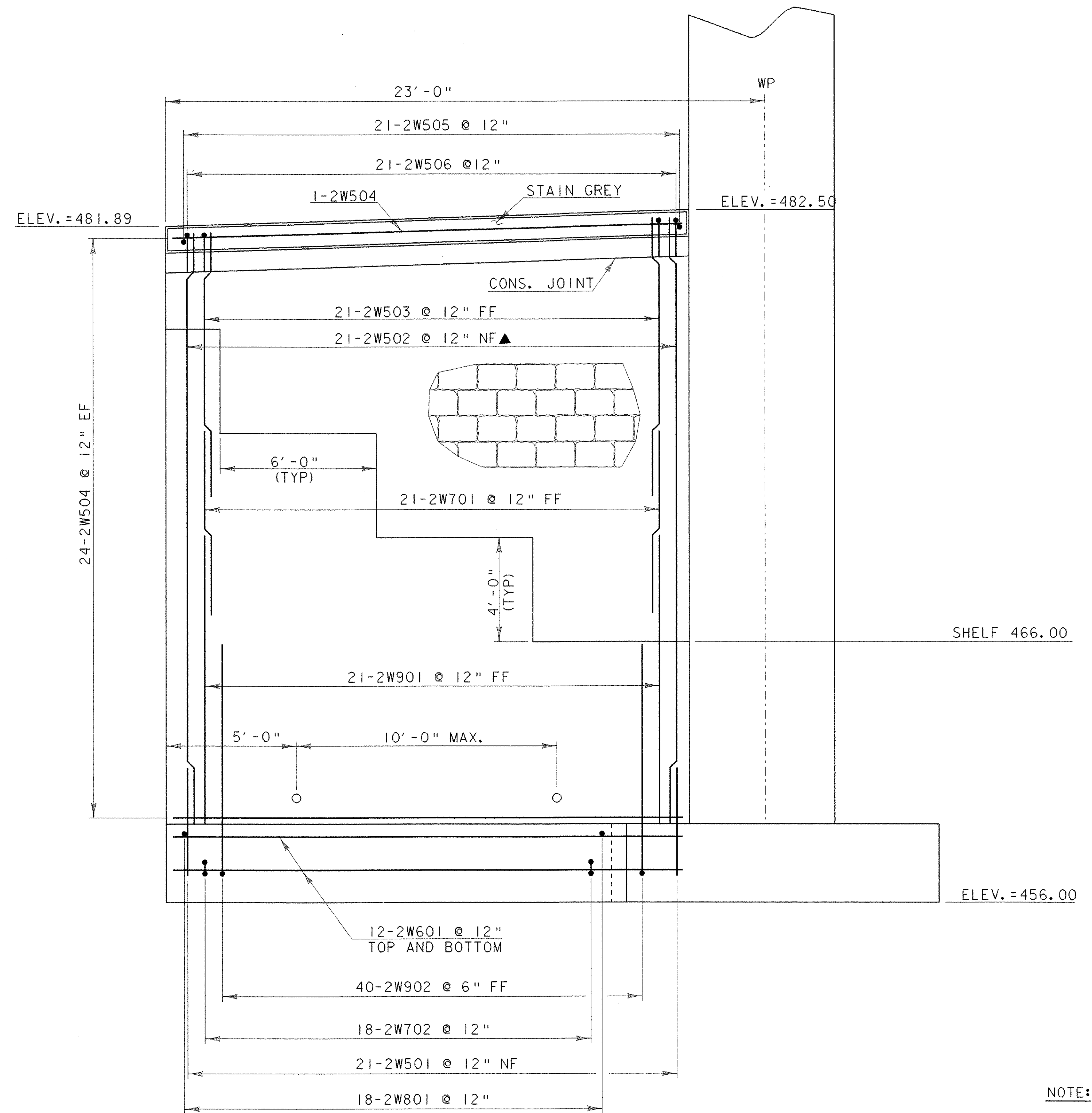
WINGWALL # 2 ELEVATION
