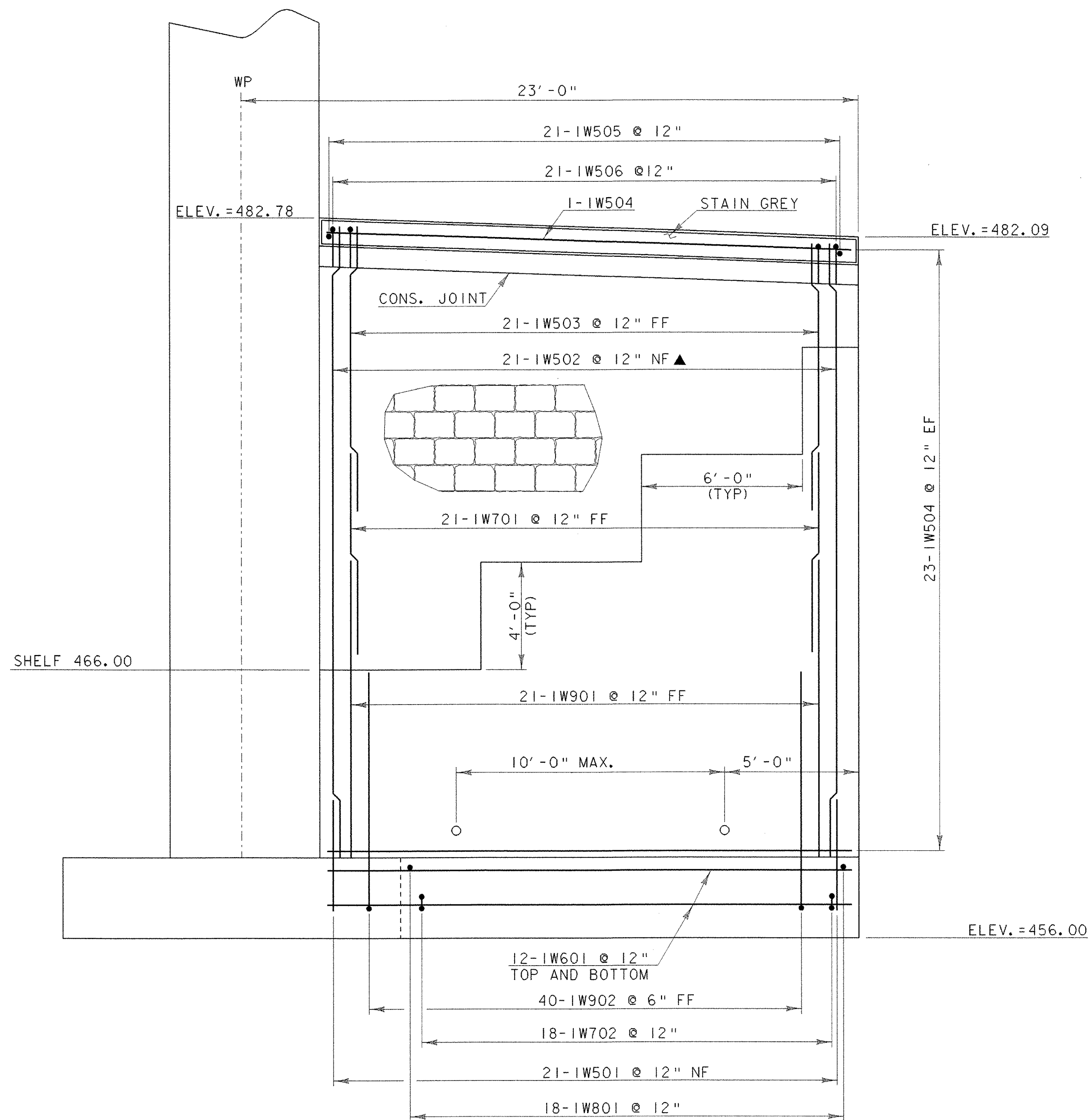
WINGWALL # 1 ELEVATION
