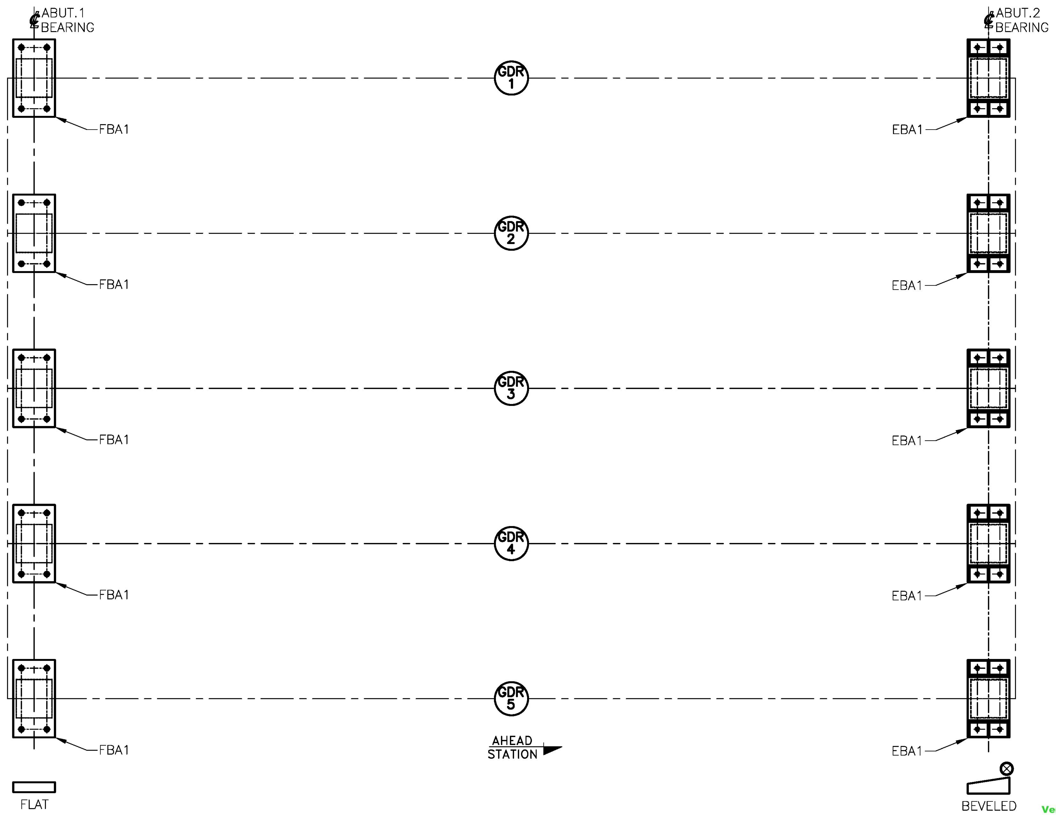
ERECTION DIAGRAM
