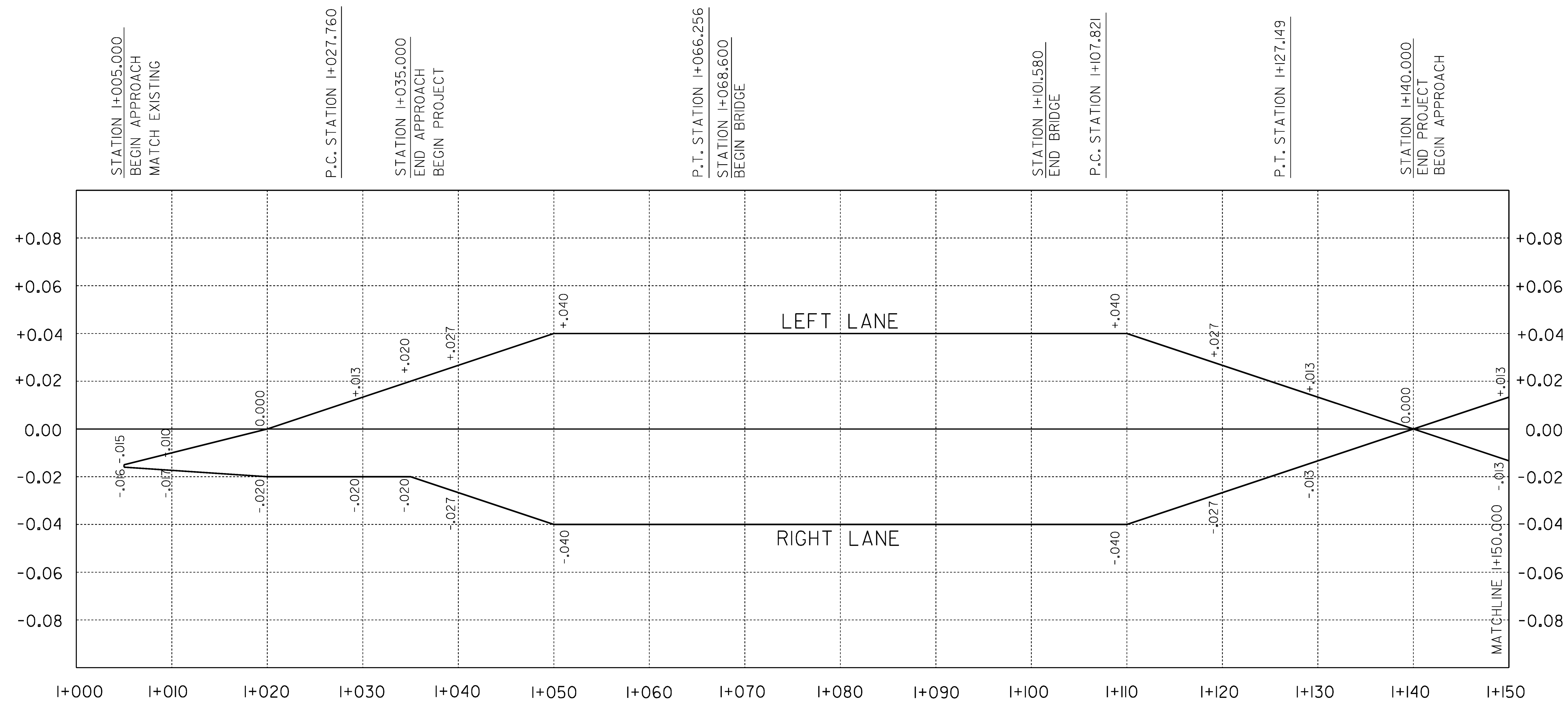
MAINLINE BANKING DIAGRAM (NOT TO SCALE)
