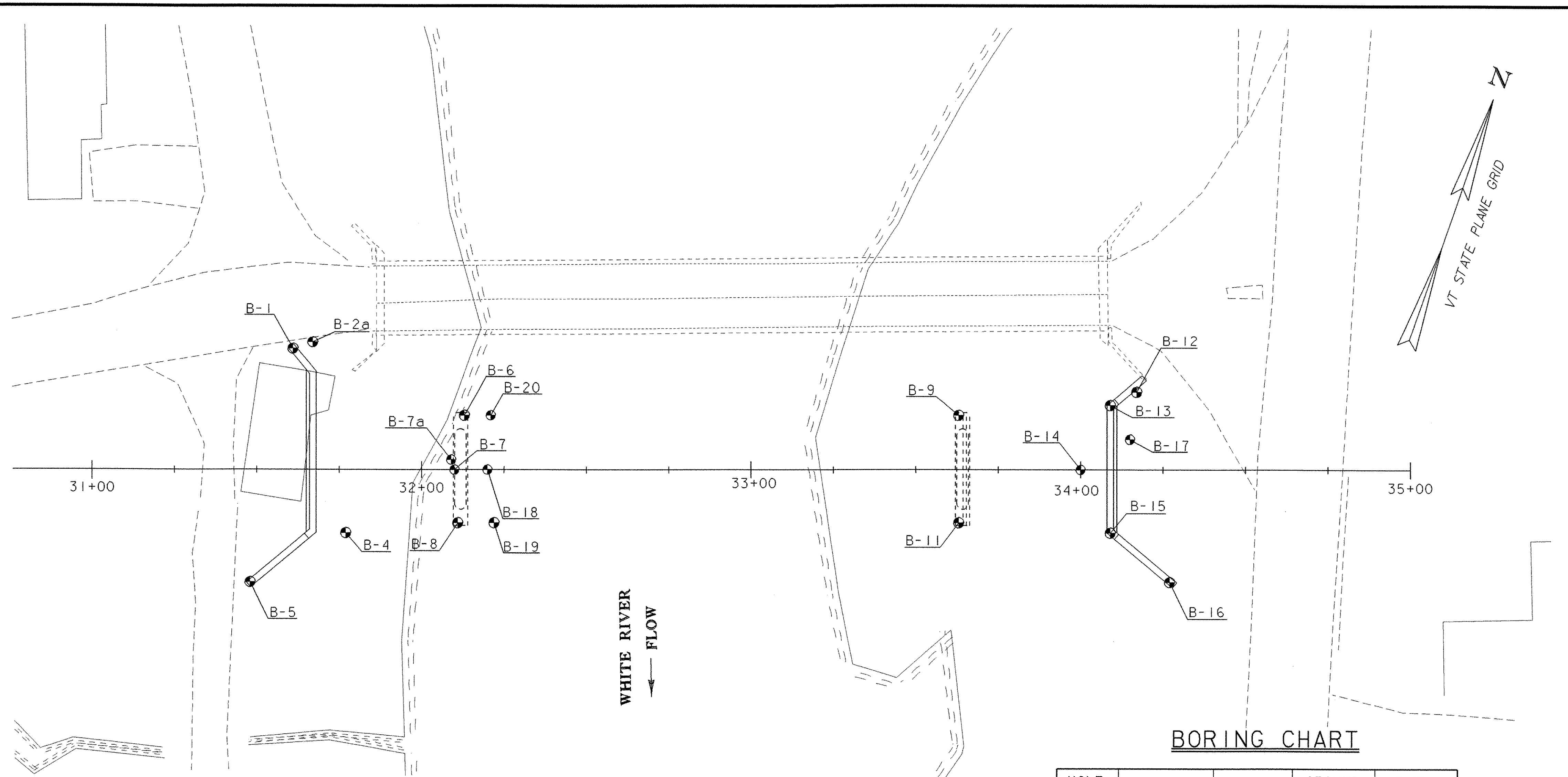
BORING CHART
