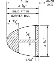
BARRIER RAIL SPLICE SECTION
