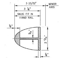
HAND RAIL SPLICE SECTION
