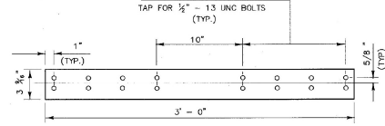
ELEVATION OF STD. BARRIER RAIL SPLICE BAR
