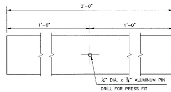
ELEVATION OF HAND RAIL SPLICE BAR
