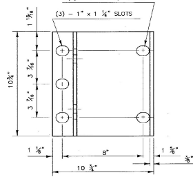
POST BASE PLAN
