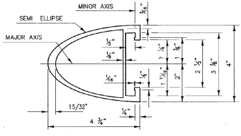
BARRIER RAIL SECTION
