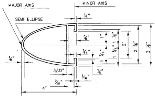
HAND RAIL SECTION
