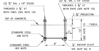
POST ANCHOR ASSEMBLY
