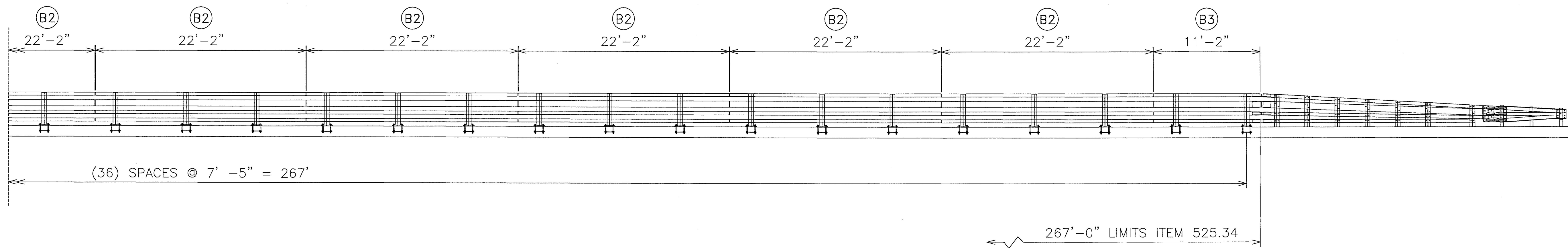
B.I.N. 57 TYPICAL RAILING ELEVATION LOOKING AT FACE OF RAIL FROM CENTERLINE OF ROAD
