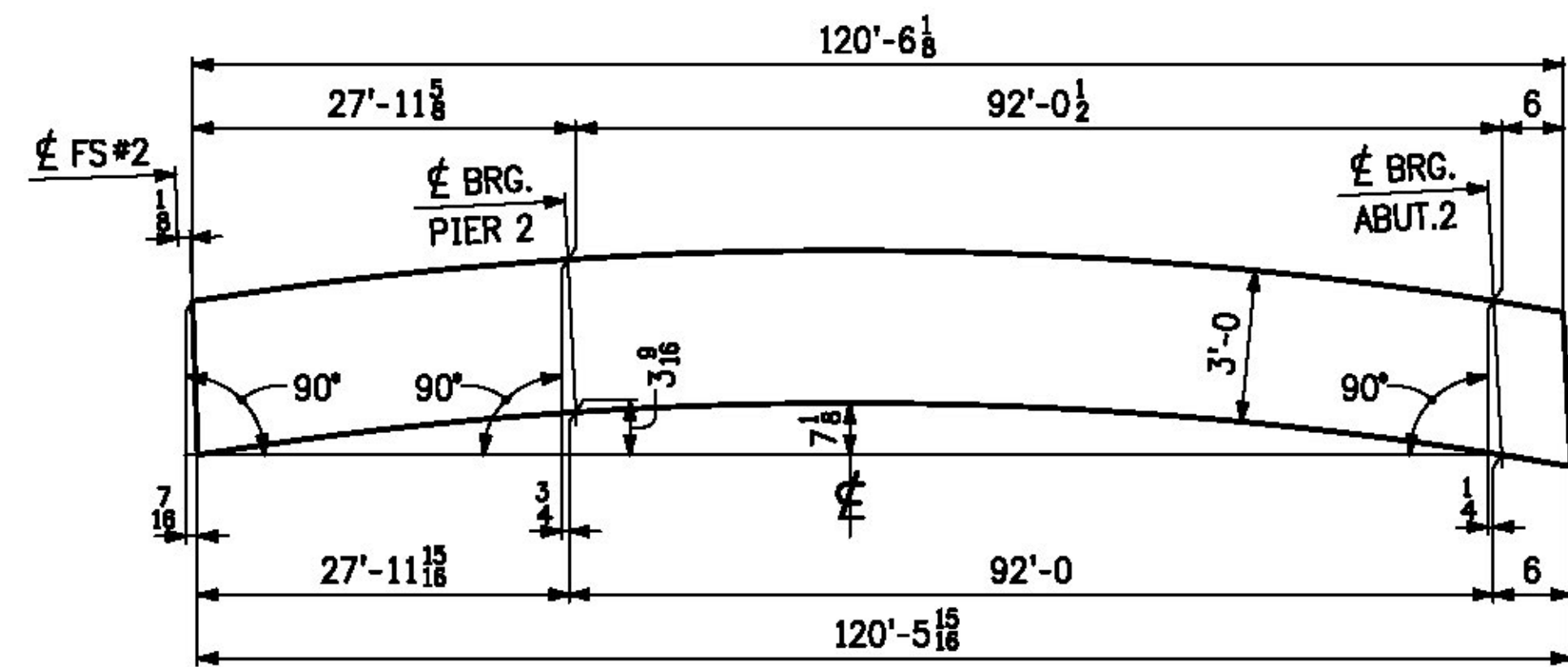
CAMBER DIAGRAM
