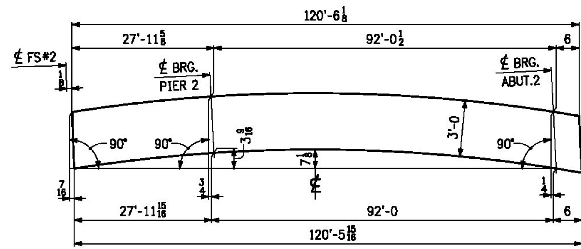
CAMBER DIAGRAM
