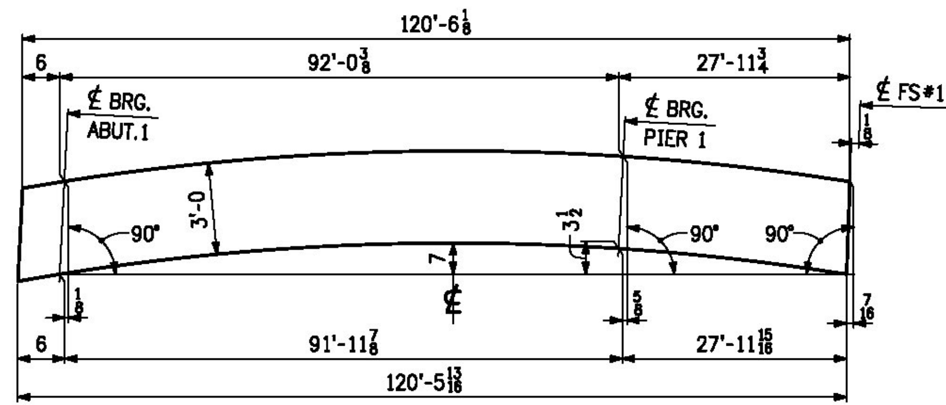
CAMBER DIAGRAM
