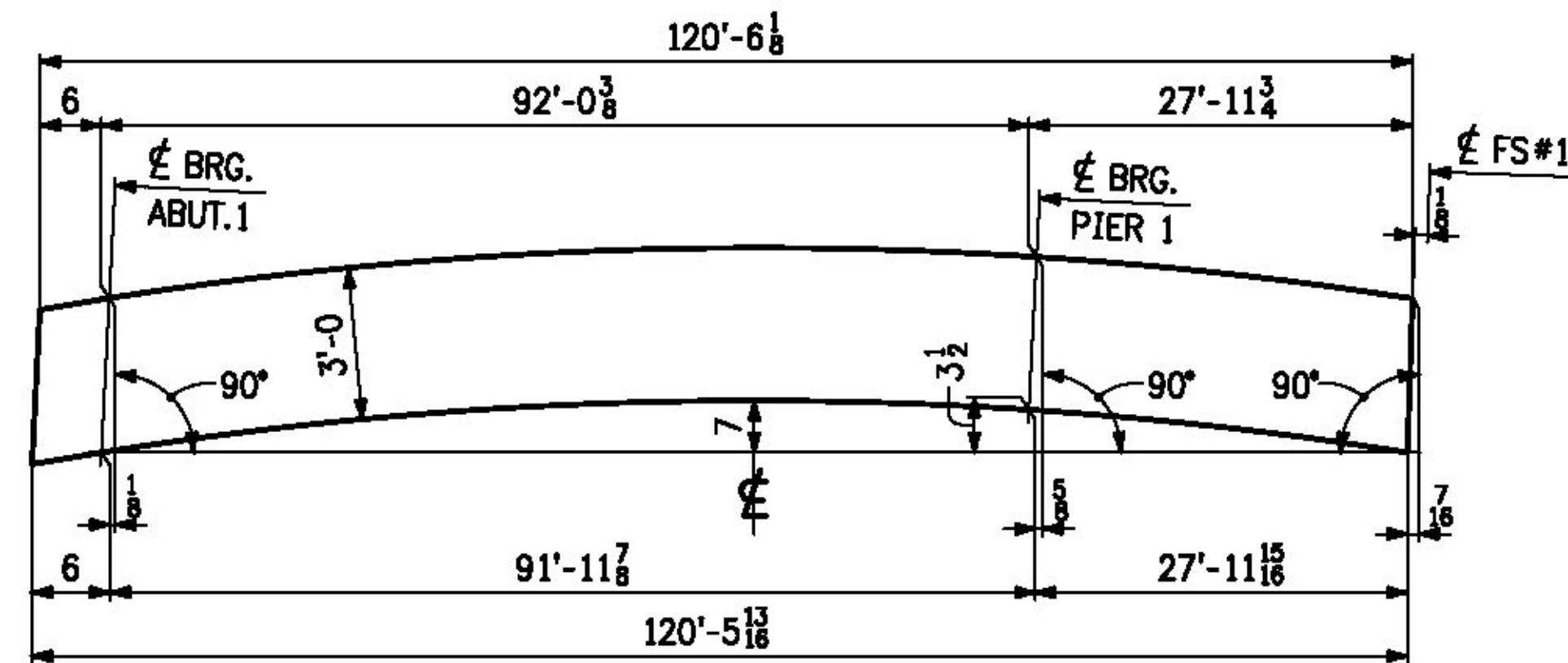
CAMBER DIAGRAM
