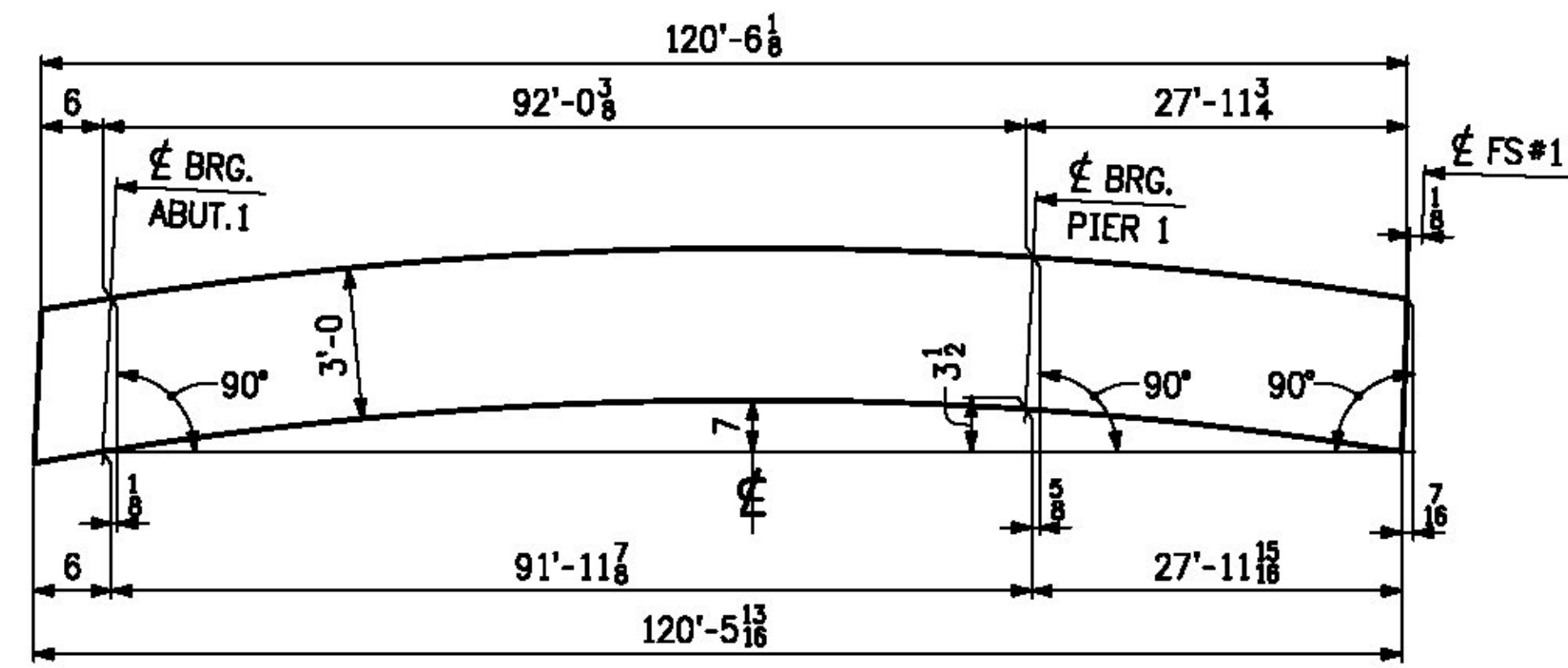
CAMBER DIAGRAM
