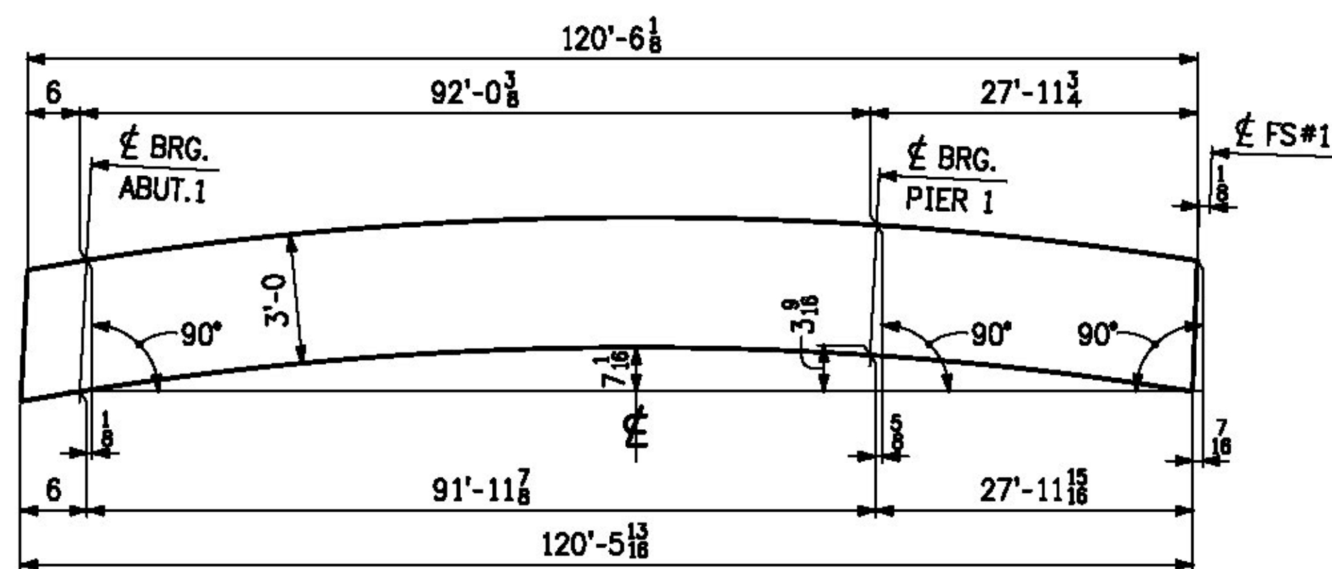
CAMBER DIAGRAM
