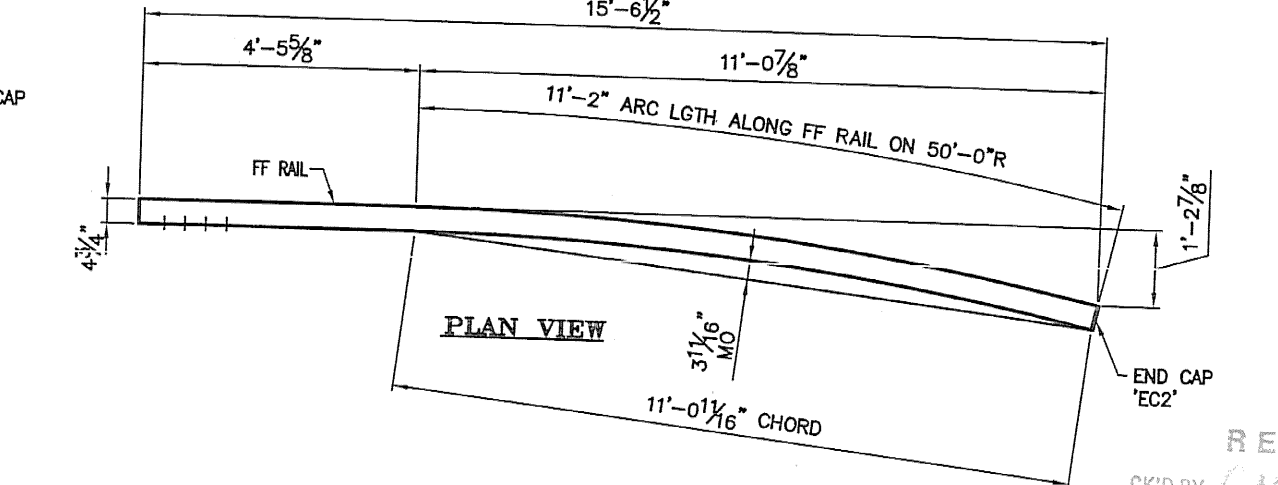
ONE REQ'D - BENT BARRIER RAIL 'MR2' (15'-7 1/8" LENGTH ALONG FF RAILING)
