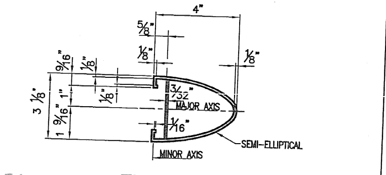
TYPICAL SECTION (BARRIER RAIL)
