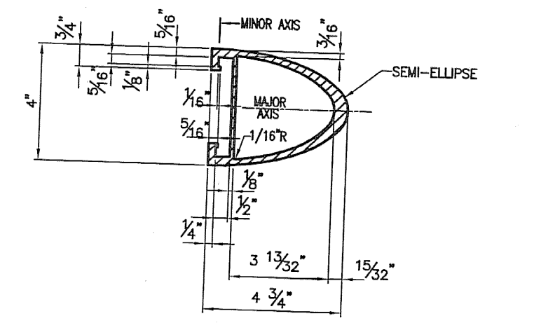
TYPICAL SECTION (BARRIER RAIL)
