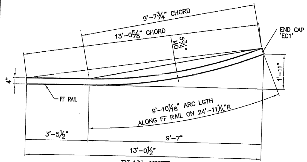
ONE REQ'D - BENT HANDRAIL 'TR2' (13'-3 9/16" LENGTH ALONG FF RAILING)
