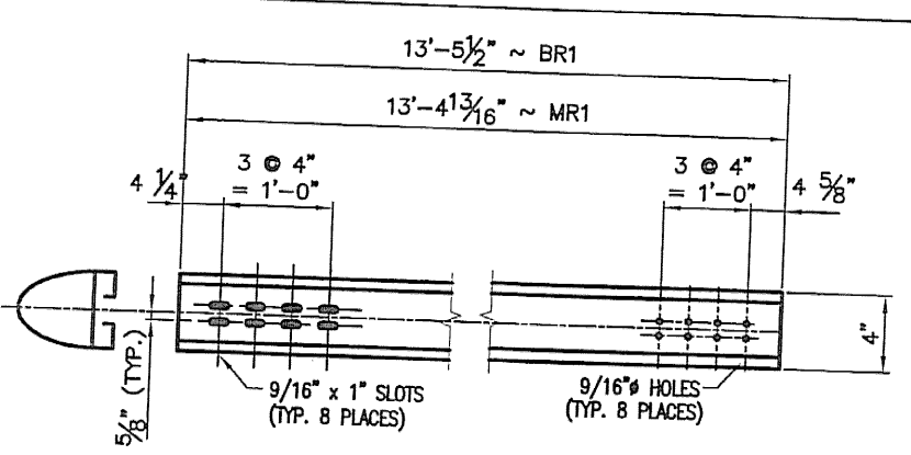
ONE REQ'D - BARRIER RAIL 'MR1' (BACK ELEVATION VIEW) ONE REQ'D - BARRIER RAIL 'BR1' (BACK ELEVATION VIEW)
