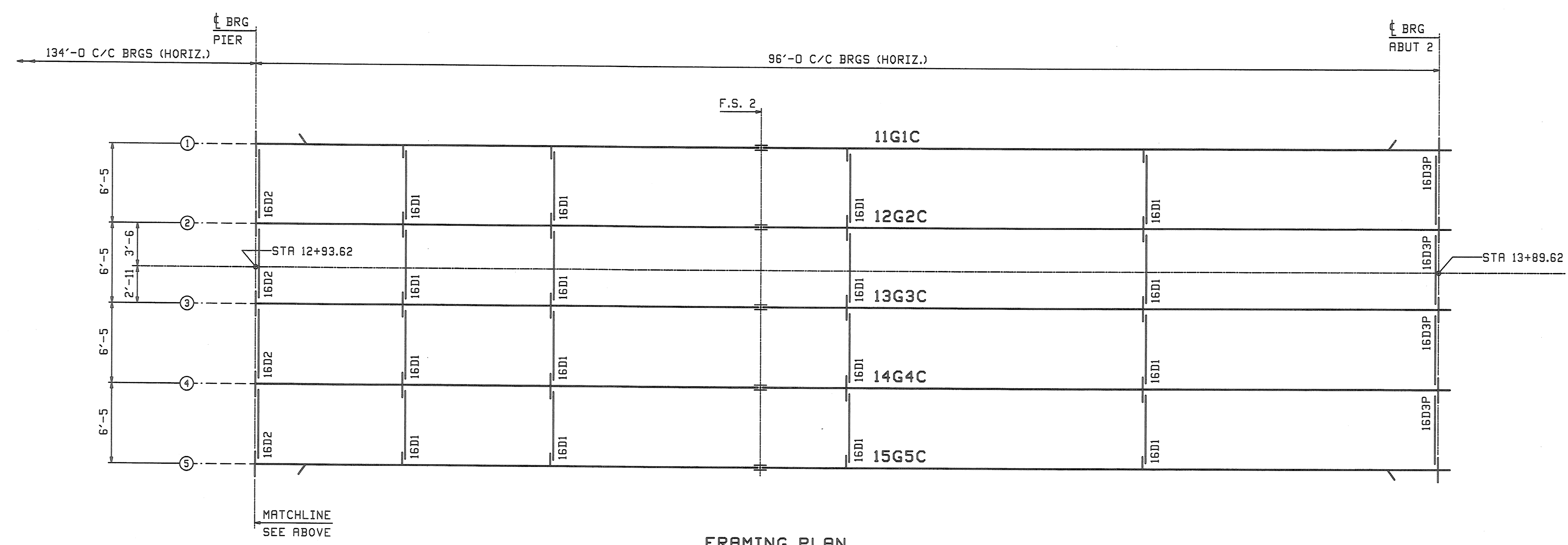
FRAMING PLAN
