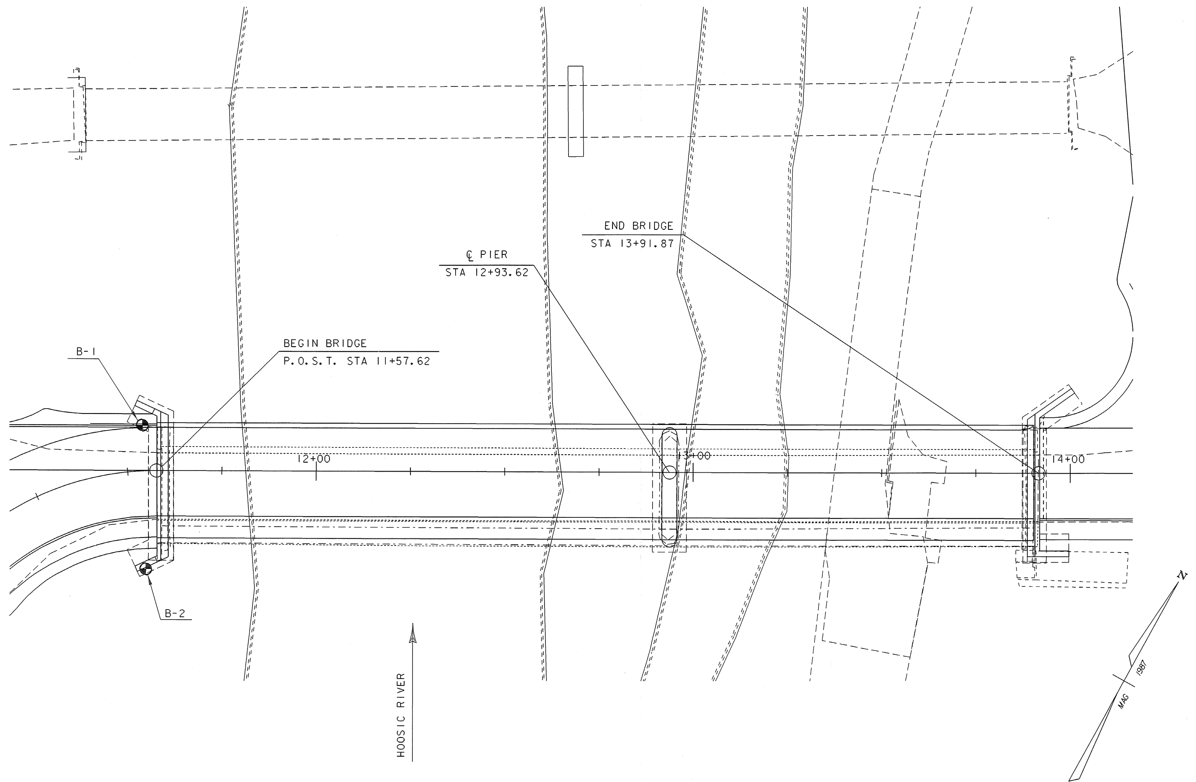
STANDARD PENETRATION BORINGS SCALE 1" = 20'-0"
