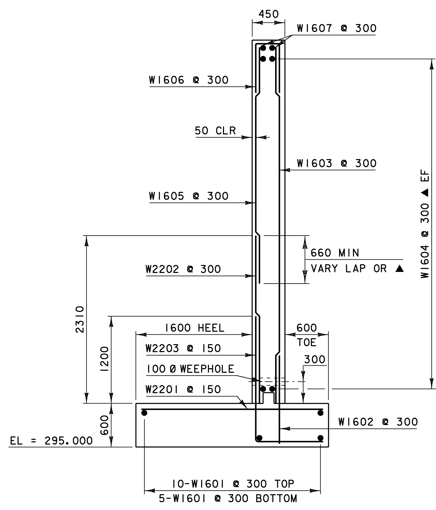
WINGWALL TYPICAL SECTION SCALE = 1:30
