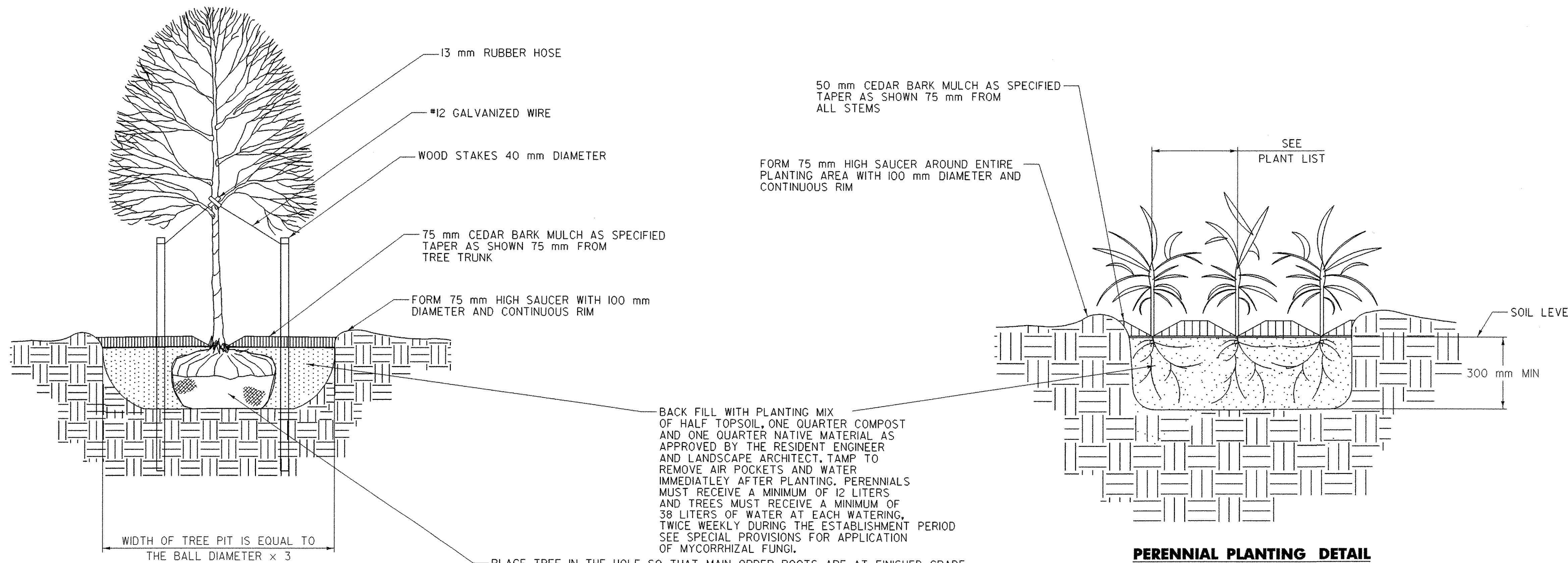
DECIDUOUS TREE PLANTING DETAIL NOT TO SCALE
