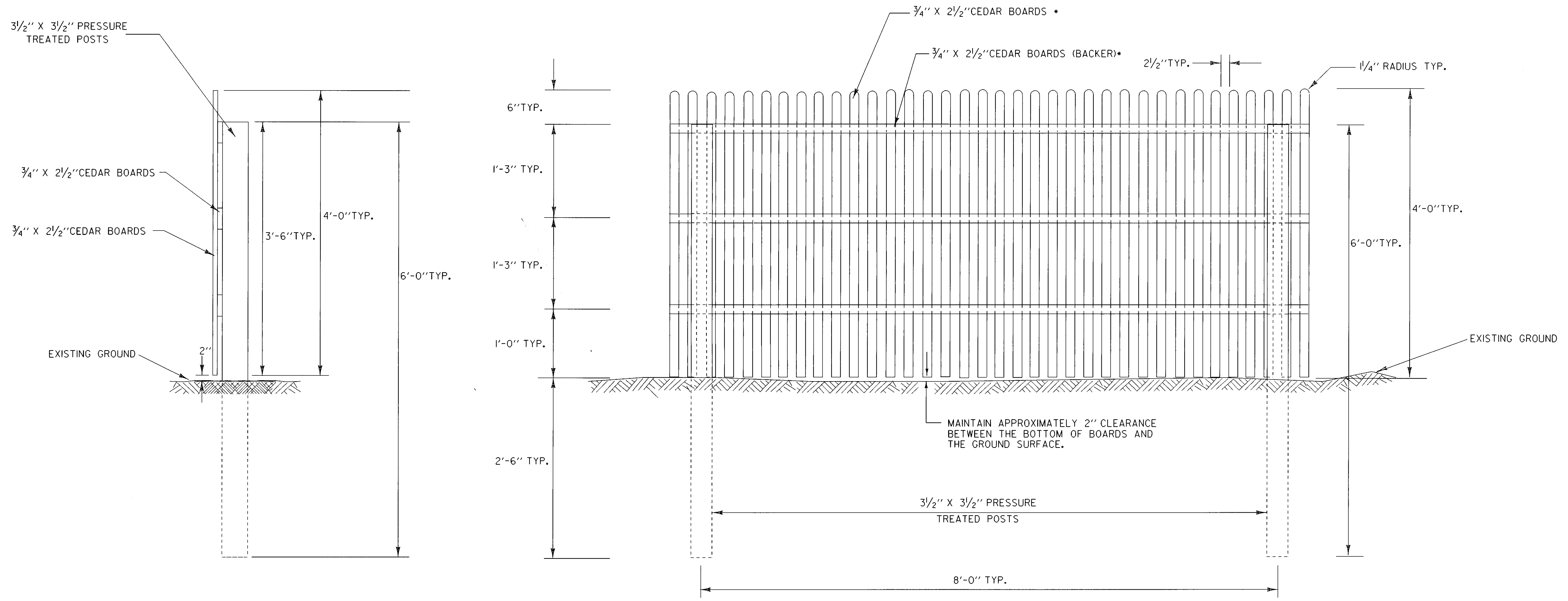
TYPICAL FENCE SECTION STATION 34+00 RT~34+82 RT
