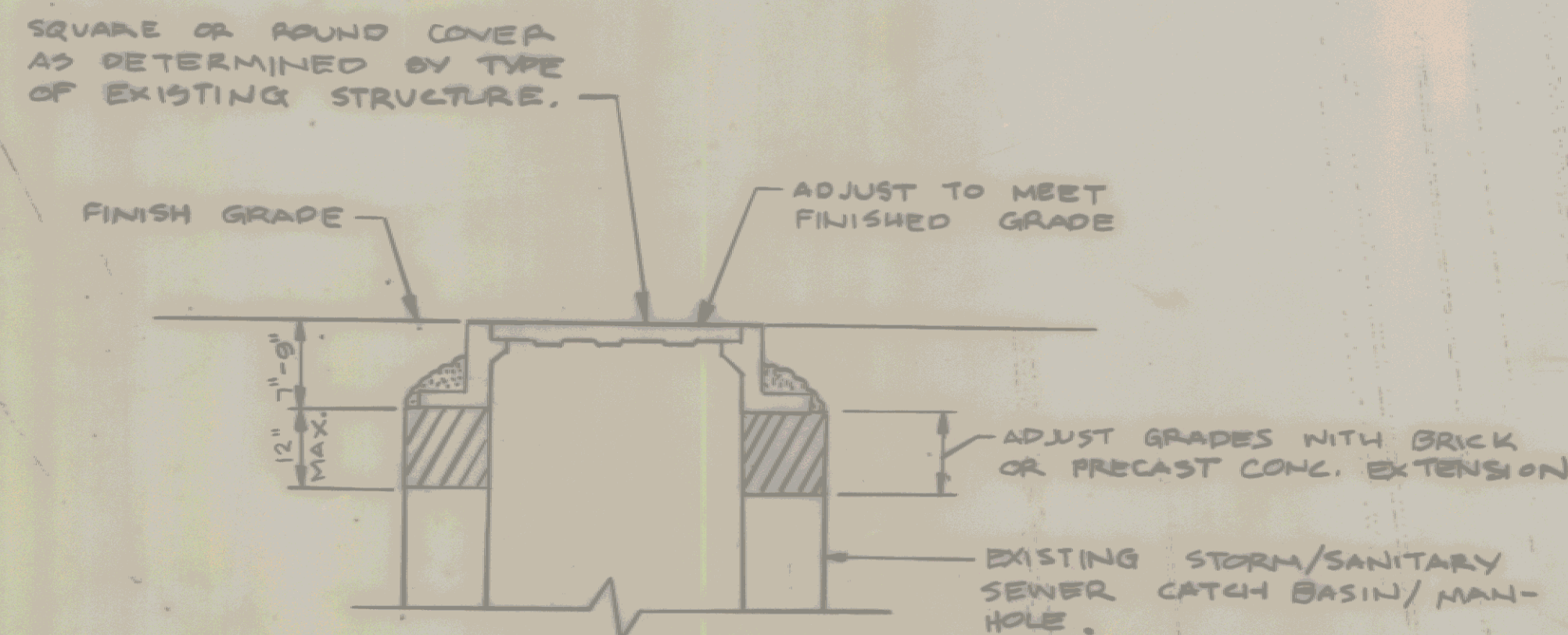
MANHOLE/CATCH BASIN COVER DETAIL NOT TO SCALE
