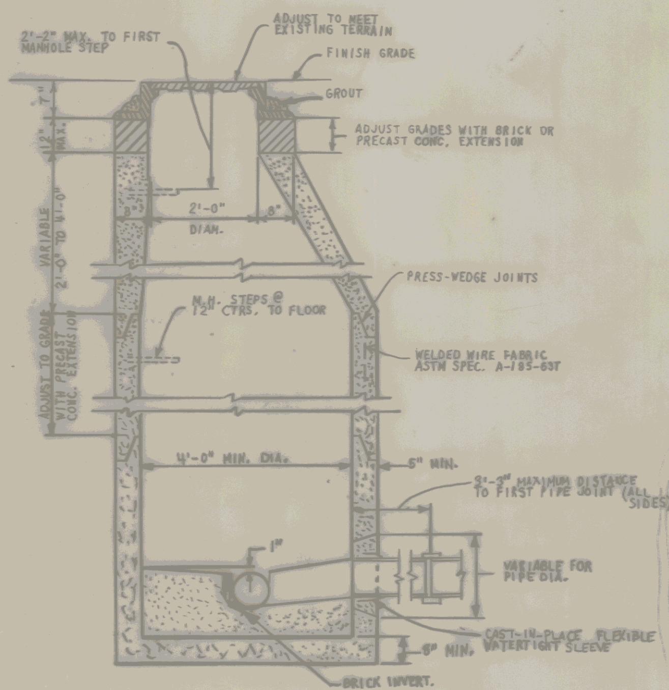
TYPICAL MANHOLE SECTION SCALE: 1/2" = 1'-0"
