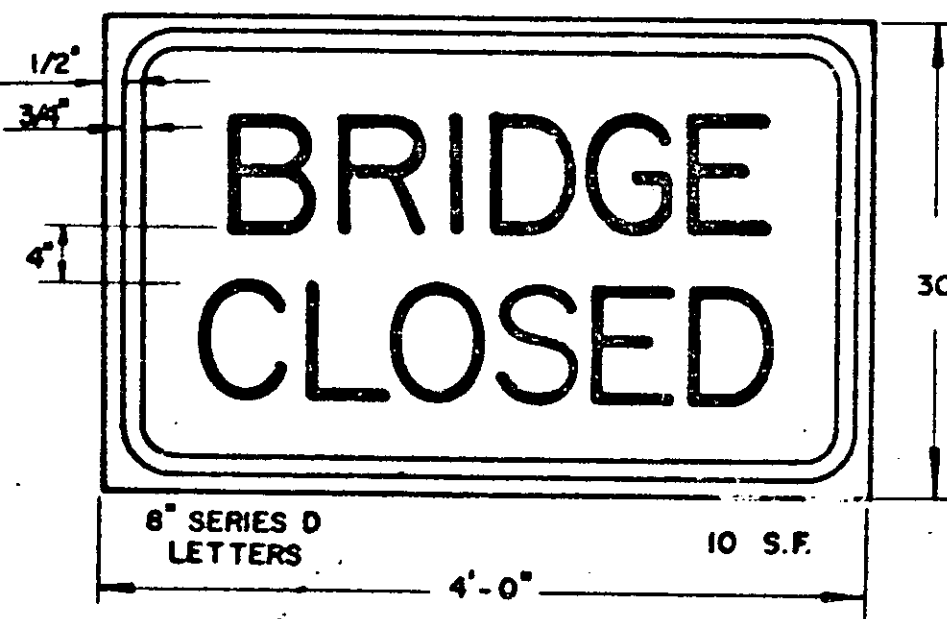
SIGN B-5 (STD. R 11-2 MODIFIED)
