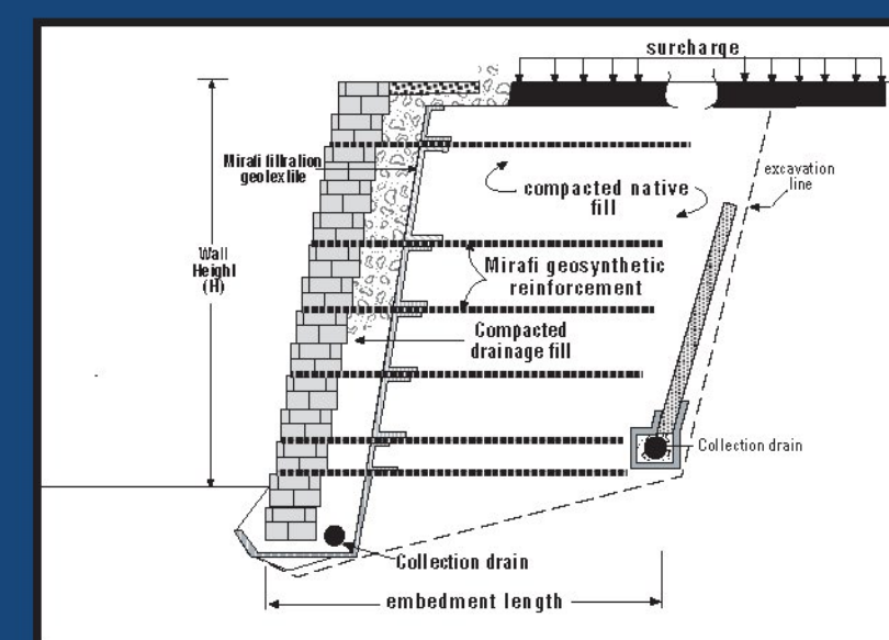
Retaining Wall
