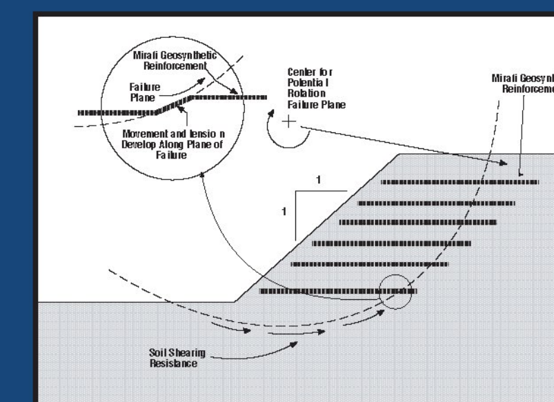
Steepened Slope
