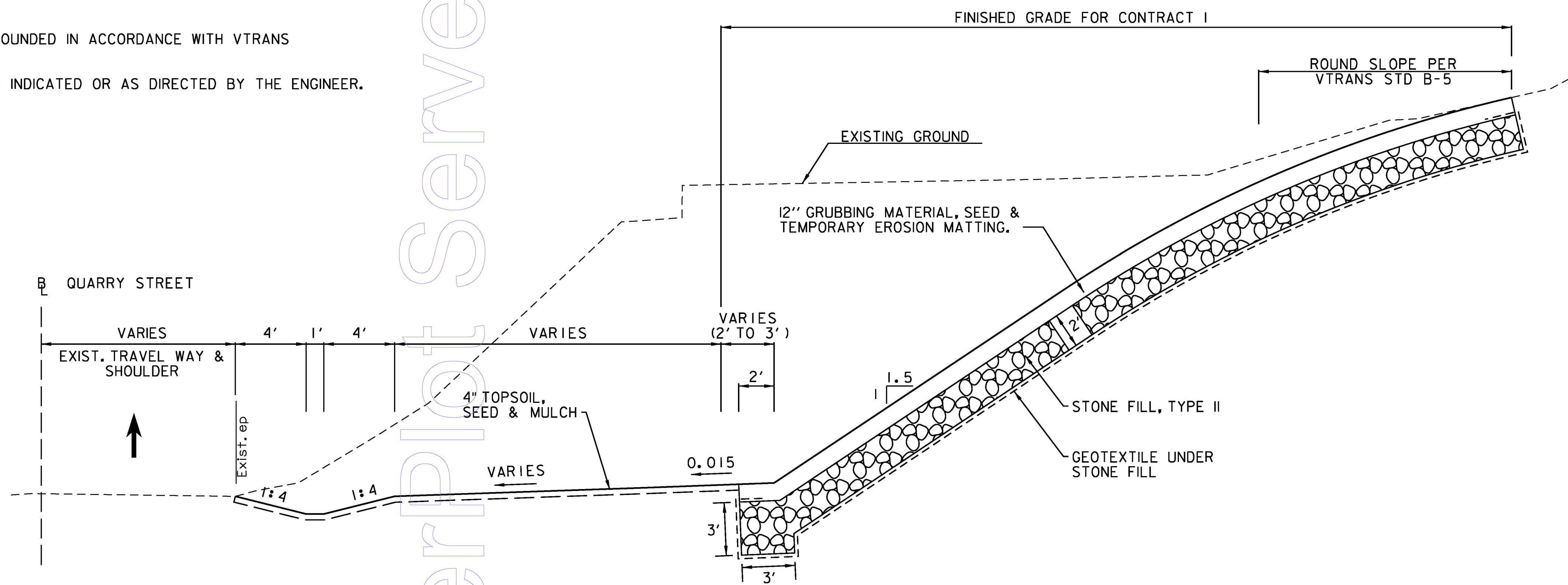
QUARRY STREET SLOPE EXCAVATION
