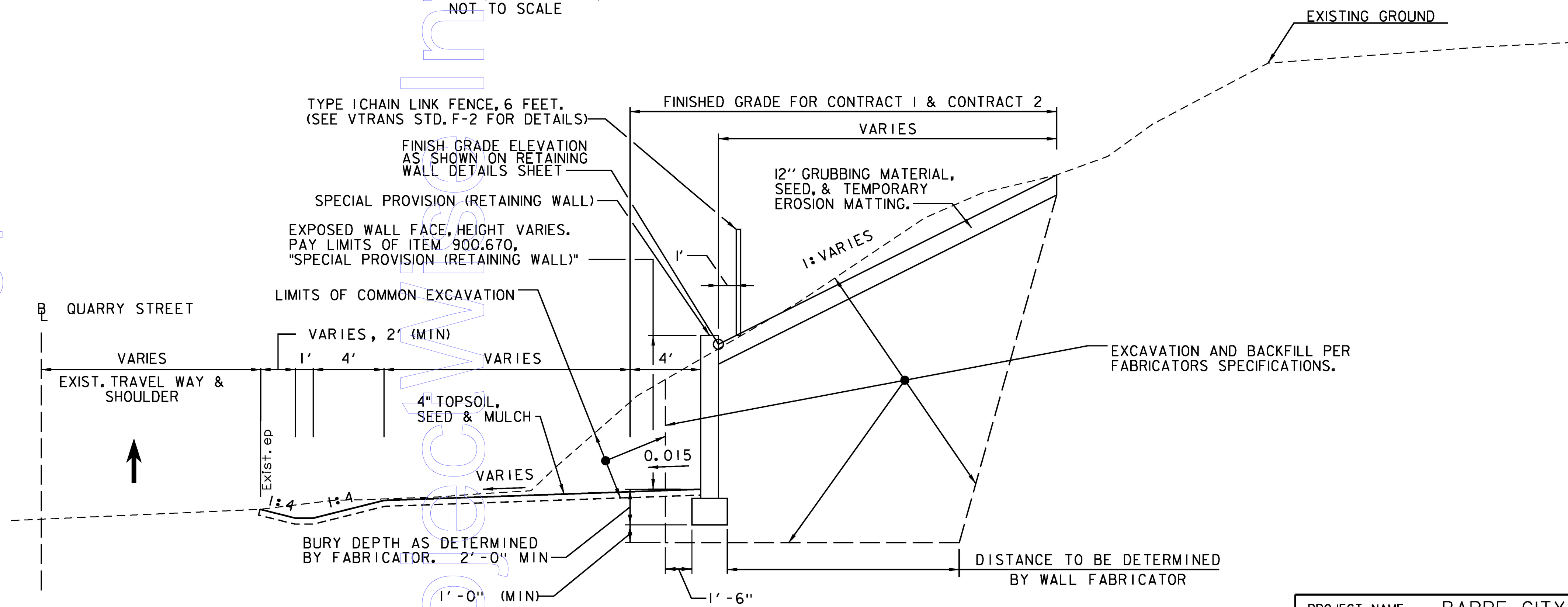
QUARRY STREET RETAINING WALL
