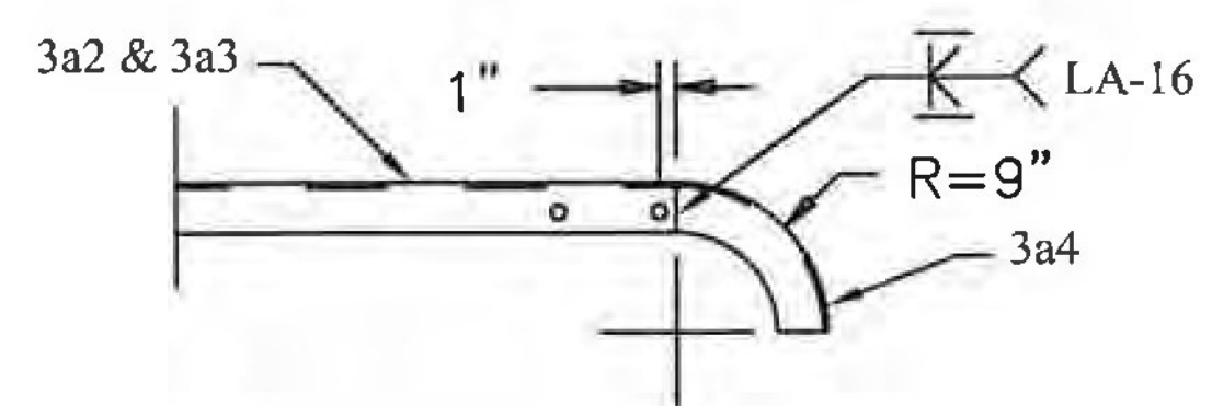
SPlice DETAIL
