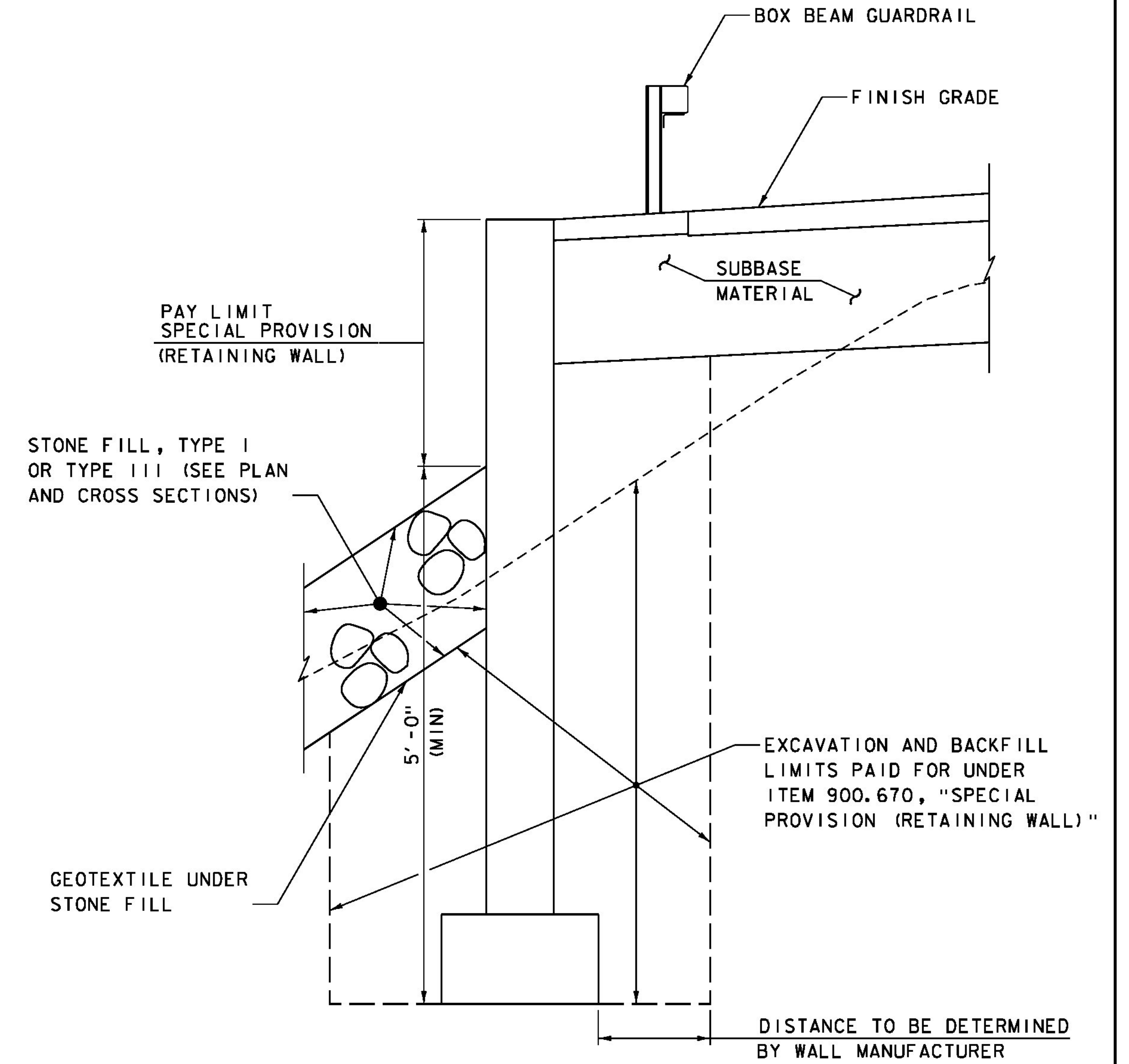
TYPICAL SECTION SCALE 1/2" = 1'-0"
