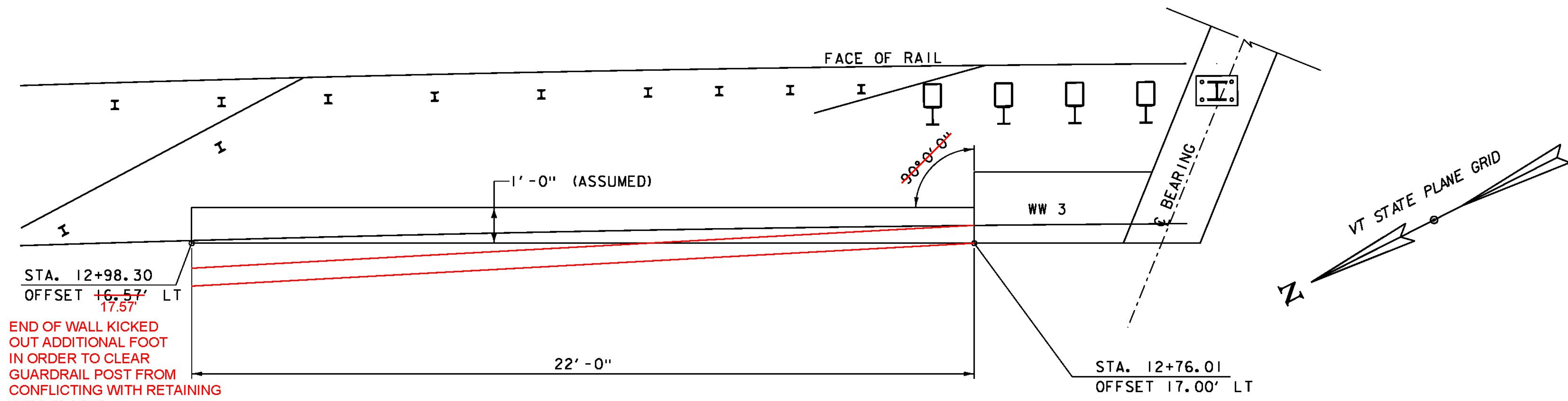
RETAINING WALL PLAN SCALE 1/2" = 1'-0"
