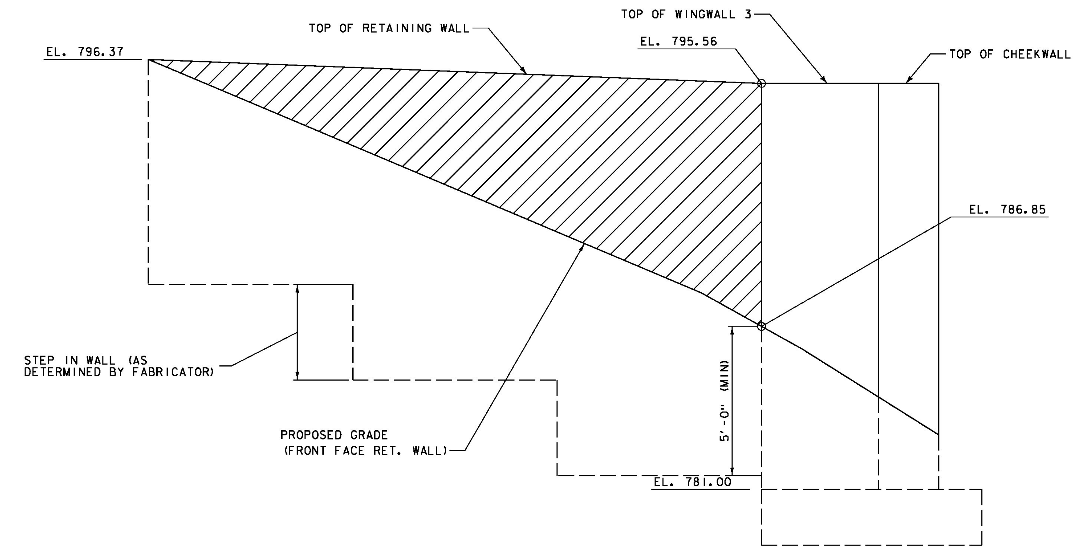
RETAINING WALL ELEVATION SCALE 1/2" = 1'-0"
