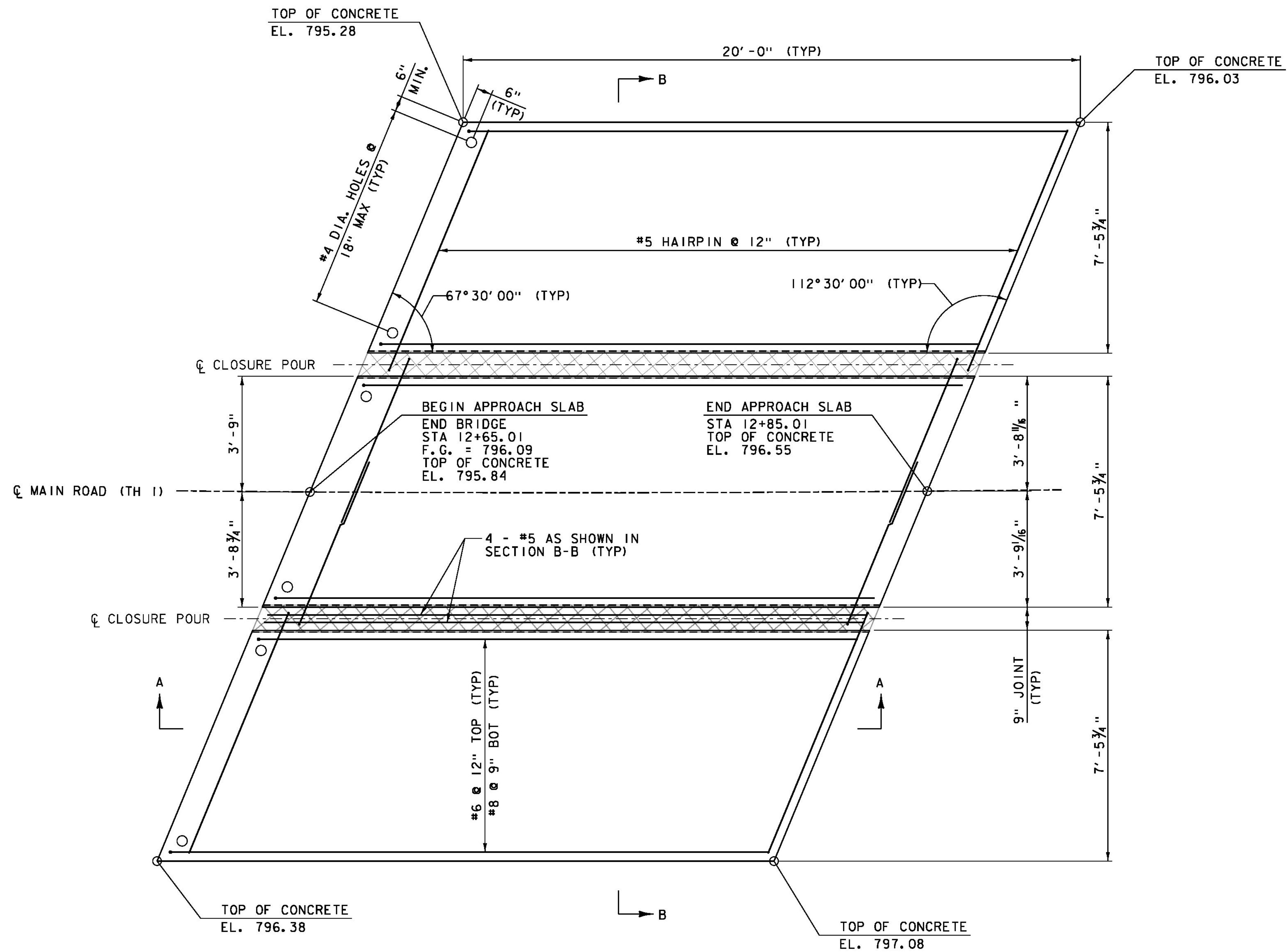
APPROACH SLAB NO 2 PLAN SCALE 1/2" = 1'-0"
