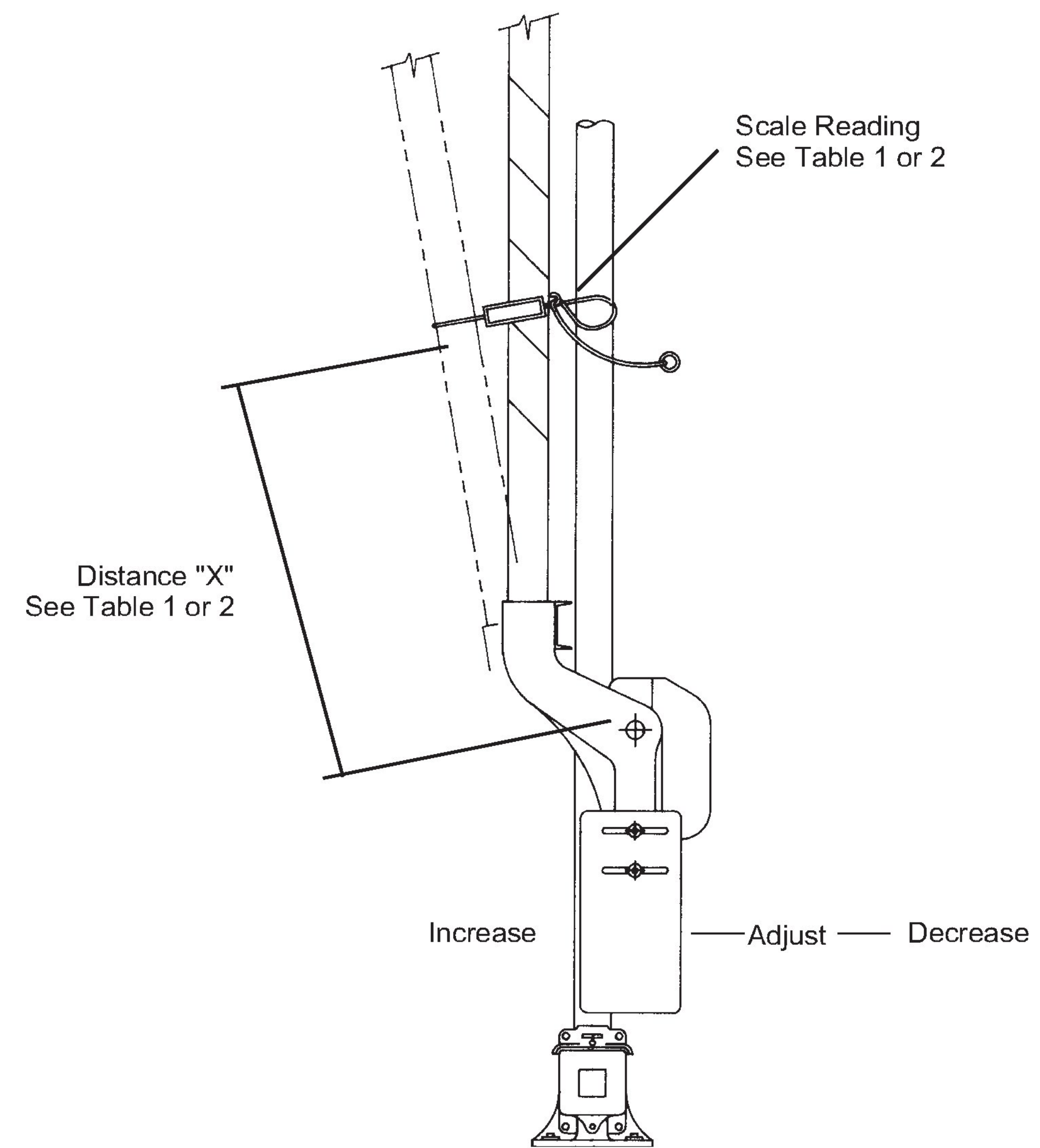
Vertical Torque Adjustment Shown with Oblong Counterweights
