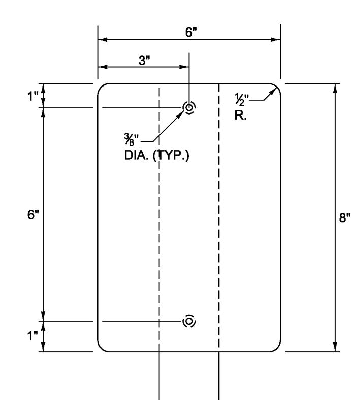
TYPE II (6'x8') DELINEATOR BACK-TO-BACK DELINEATORS WITH RETROREFLECTIVE SHEETING
