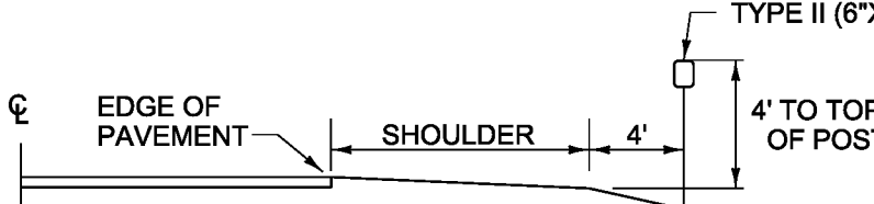
DELINEATOR PLACEMENT
