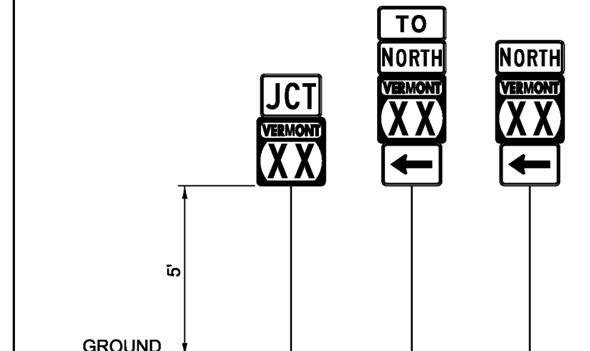
GUIDE SIGN PLACEMENT DETAIL
