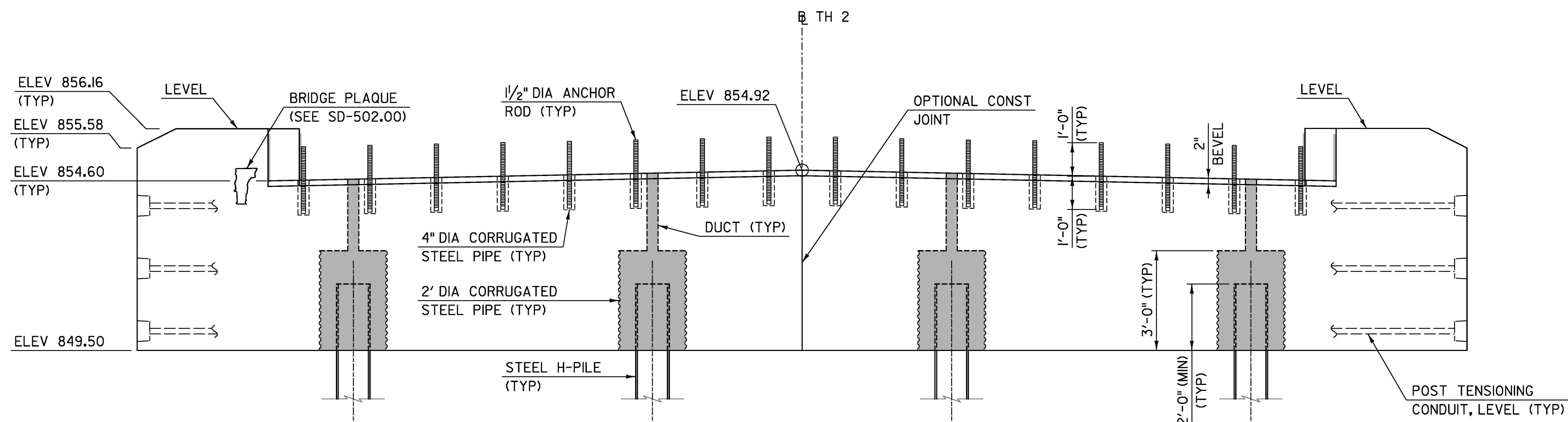
ABUTMENT NO 2 - ELEVATION SCALE: 1/2" = 1'-0"
