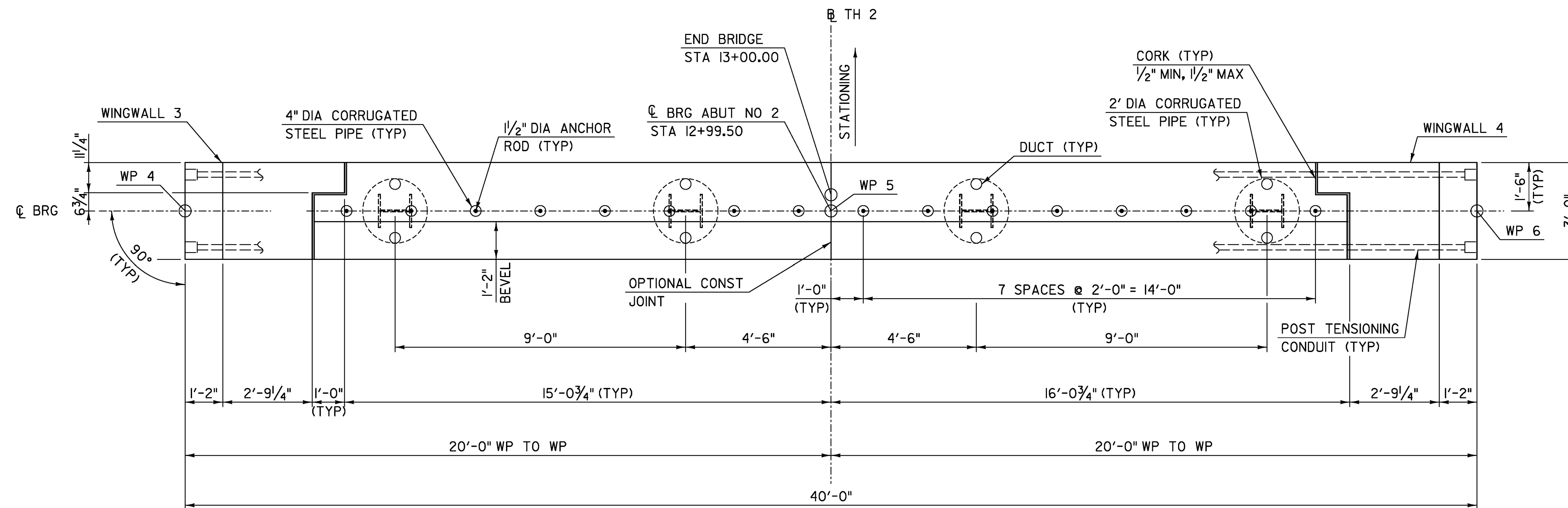
ABUTMENT NO 2 - PLAN SCALE: 1/2" = 1'-0"
