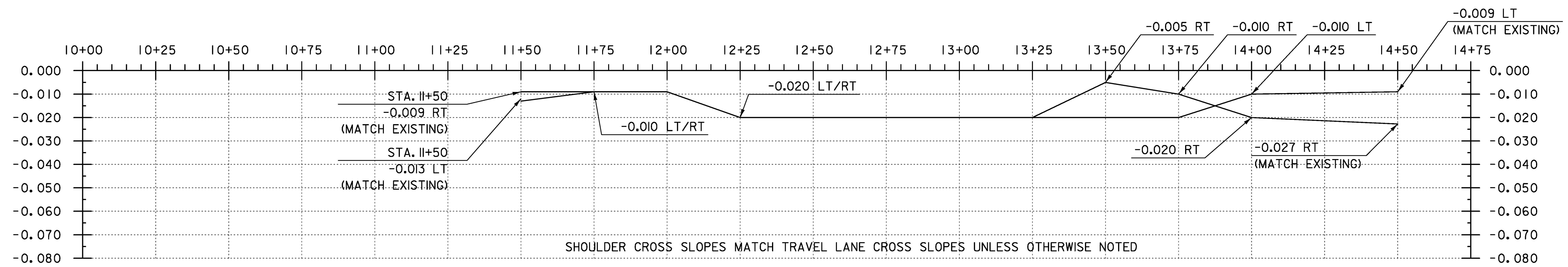
BANKING DIAGRAM - TH 2 HORIZ: 1"=20' NO VERTICAL SCALE
