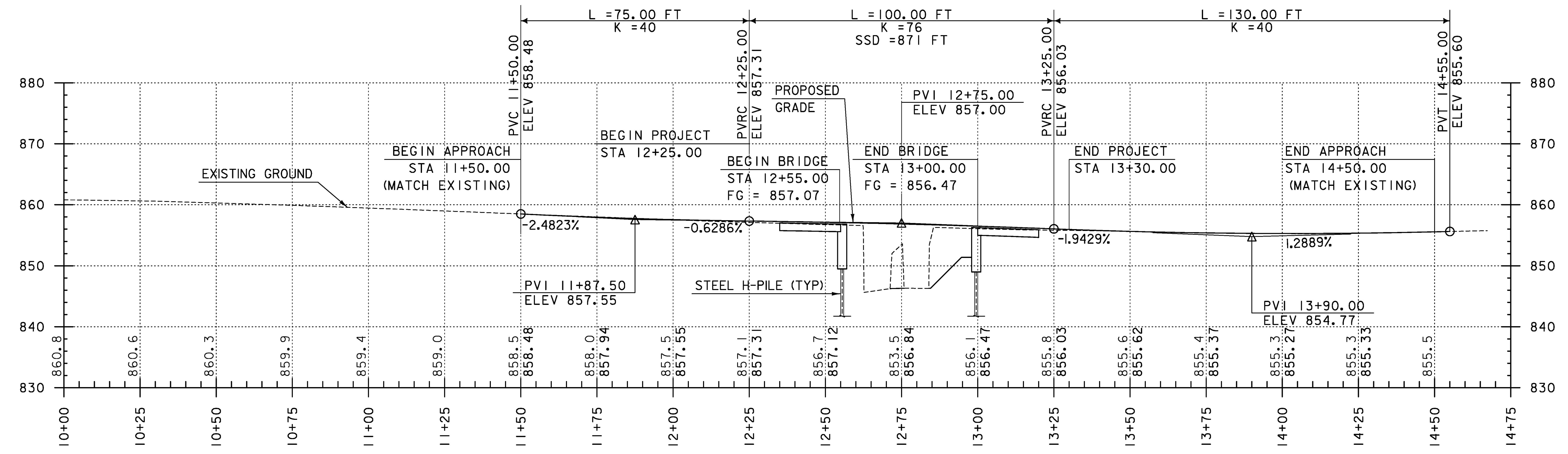
PROFILE - TH 2 SCALE: HORIZONTAL 1" = 20'-0" VERTICAL 1" = 10'-0"
