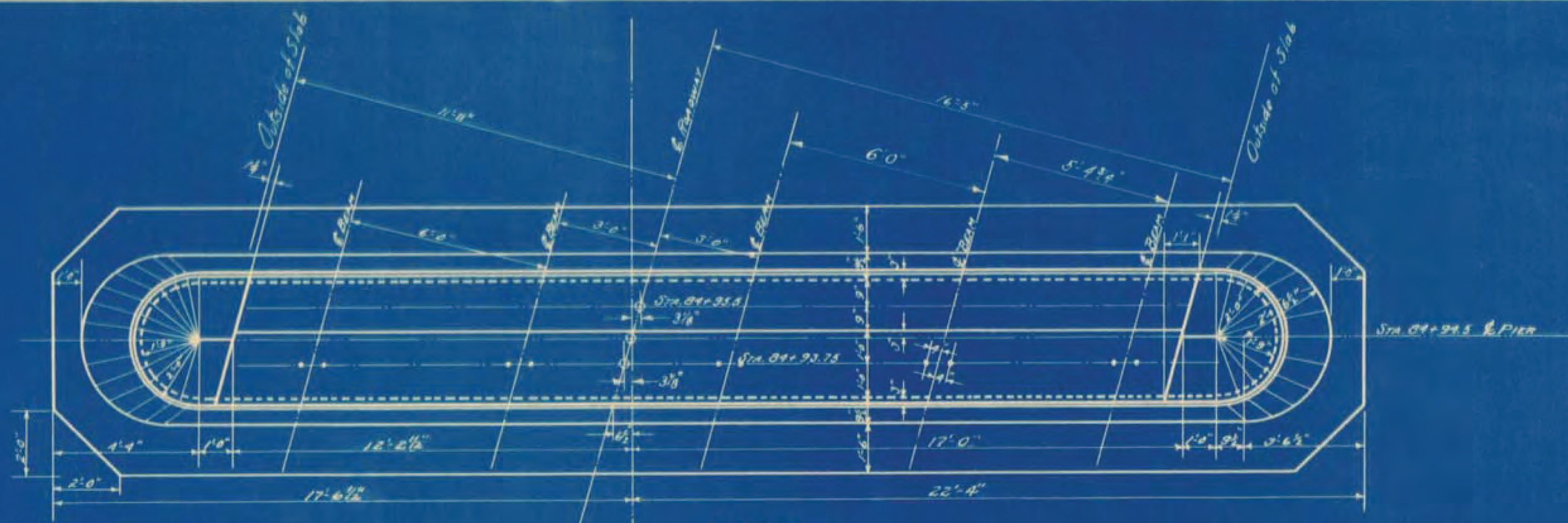
PLAN
