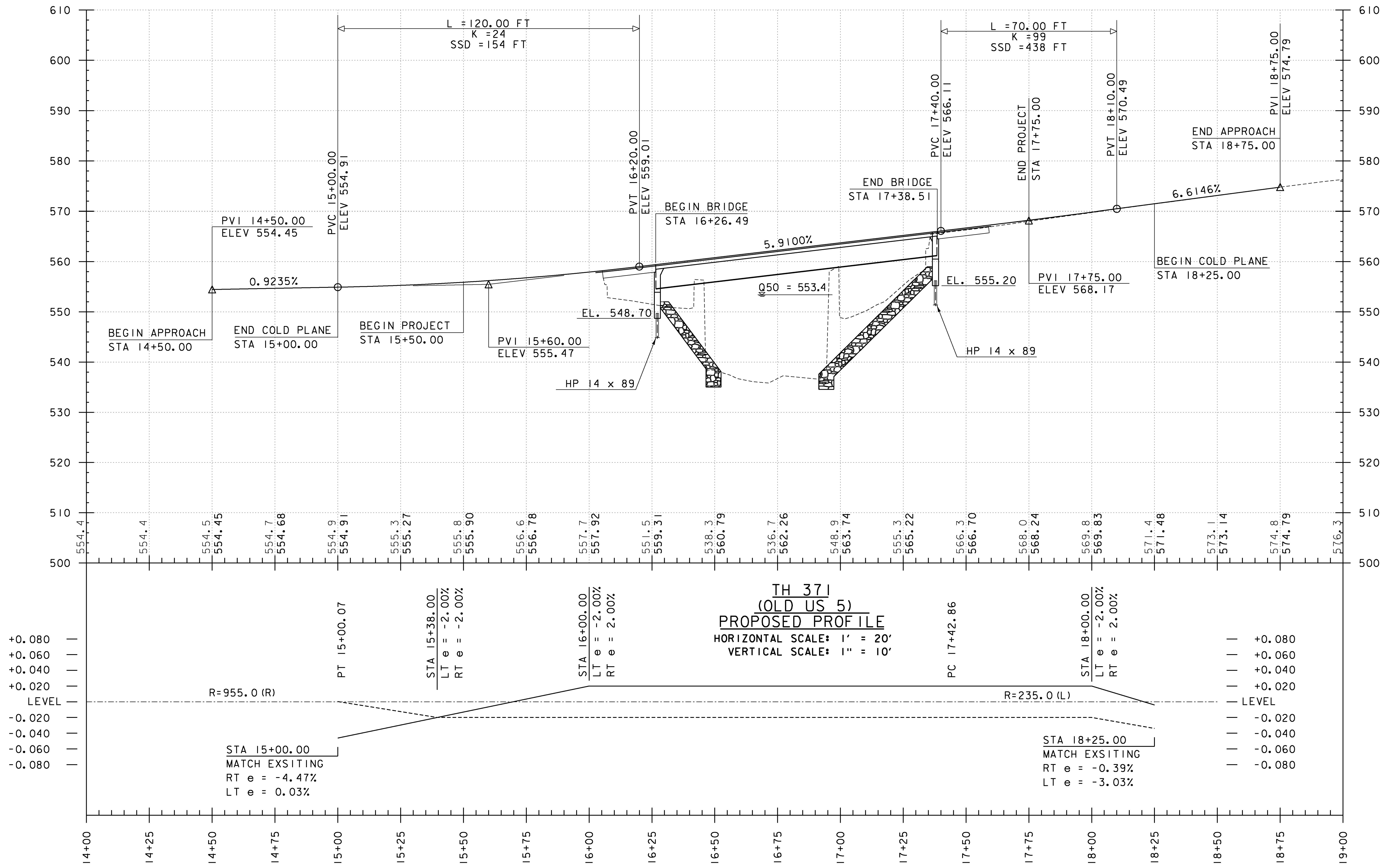
BANKING DIAGRAM HORIZONTAL SCALE: 1' = 20'
