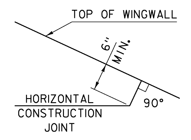
HORIZONTAL WINGWALL CONSTRUCTION JOINT (NOT TO SCALE)
