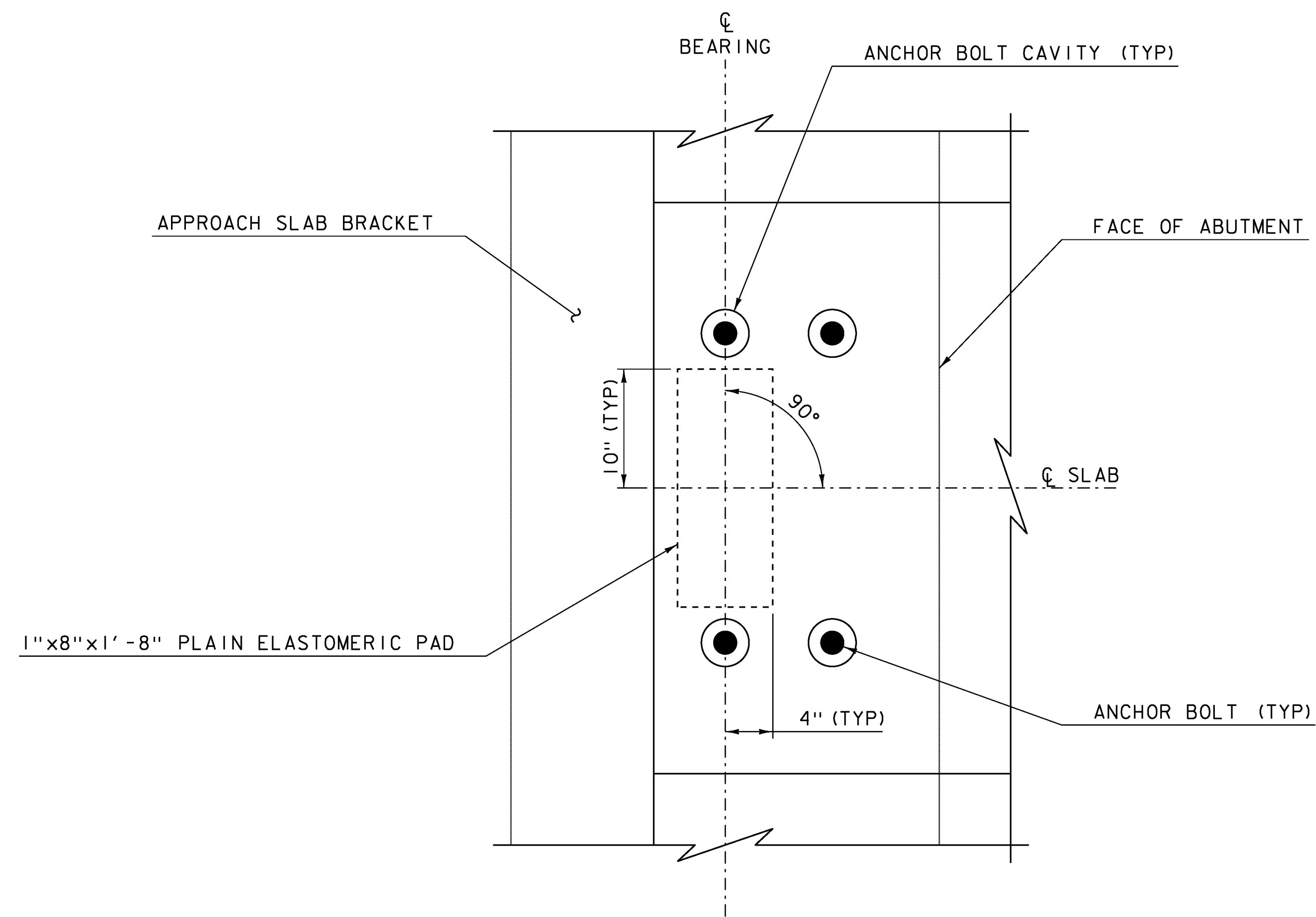
BEARING LAYOUT
