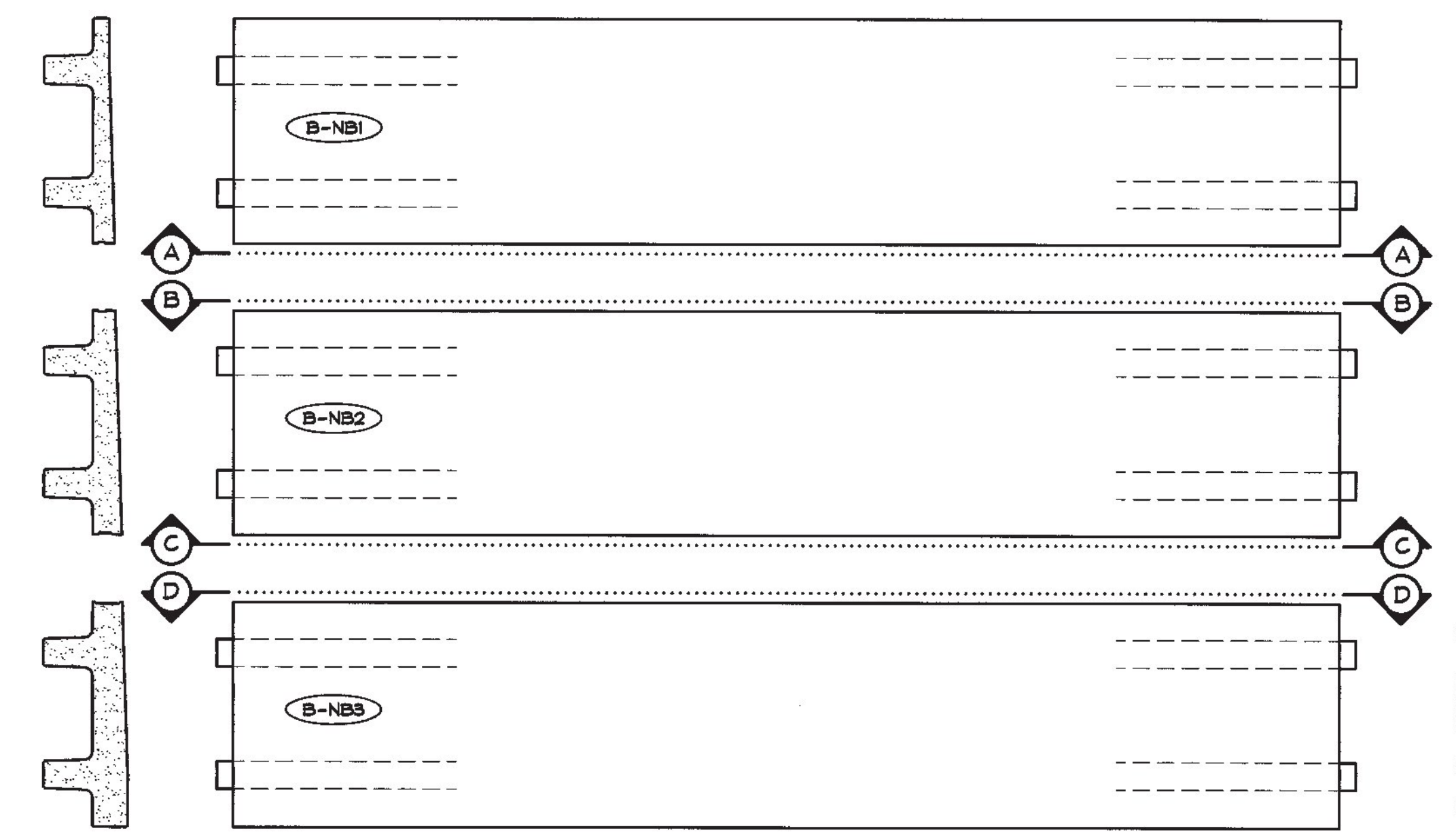
SCHEMATIC PLAN VIEW OF NEXT BEAMS N.T.S.
