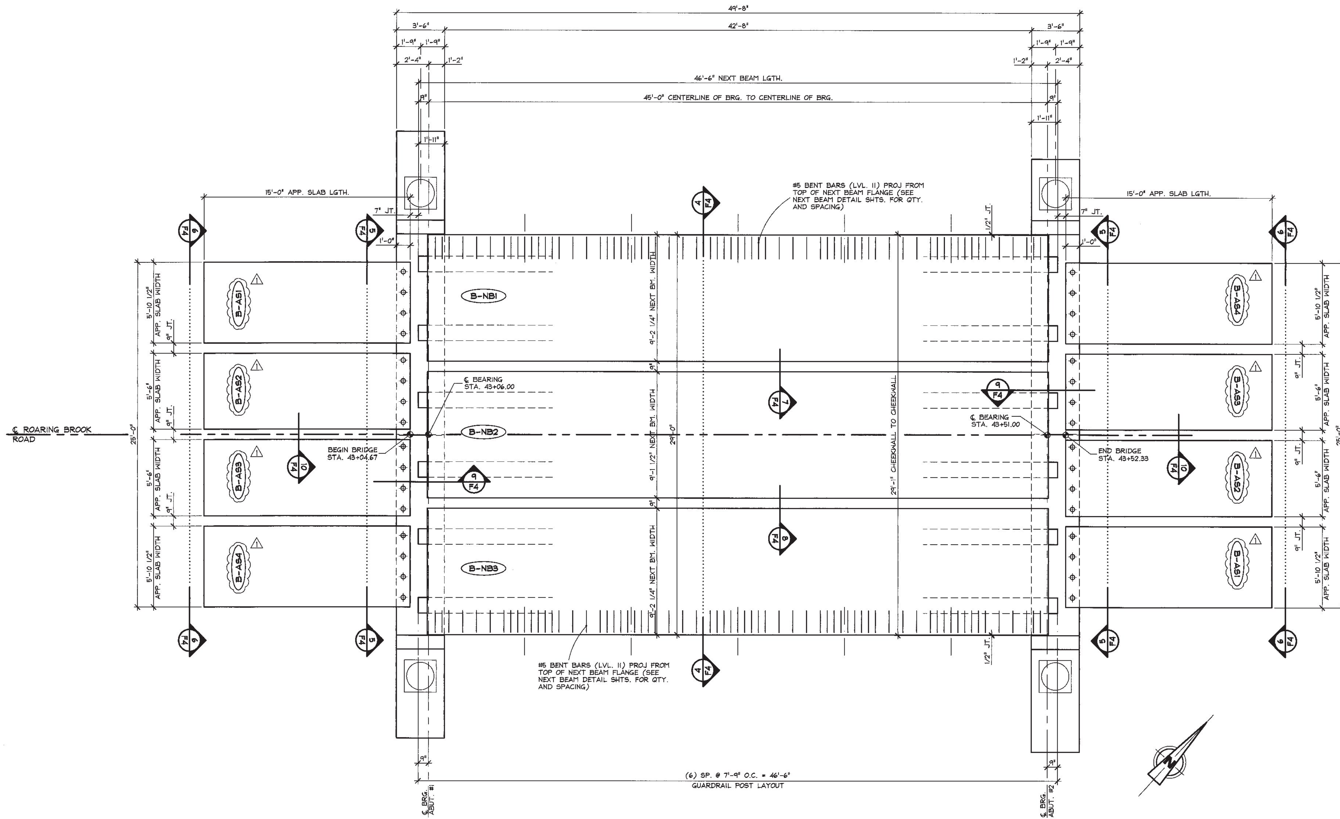
1 PRESTRESSED NEXT BEAM & APPROACH SLAB LAYOUT F3 1/4" = 1'-0"
