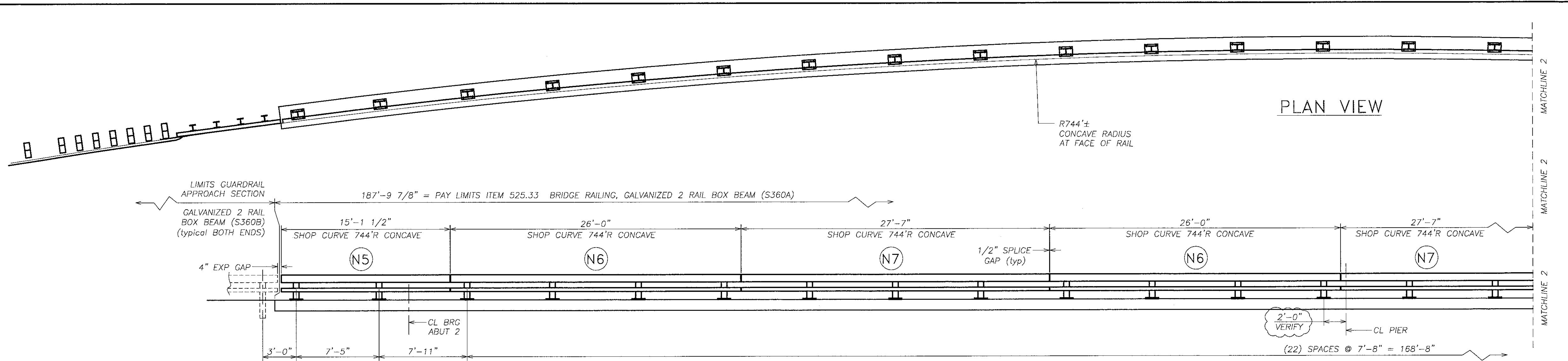
EAST SIDE RAILING ELEVATION LOOKING AT TRAFFIC FACE OF RAILING FACING EAST FROM CENTERLINE OF ROAD
