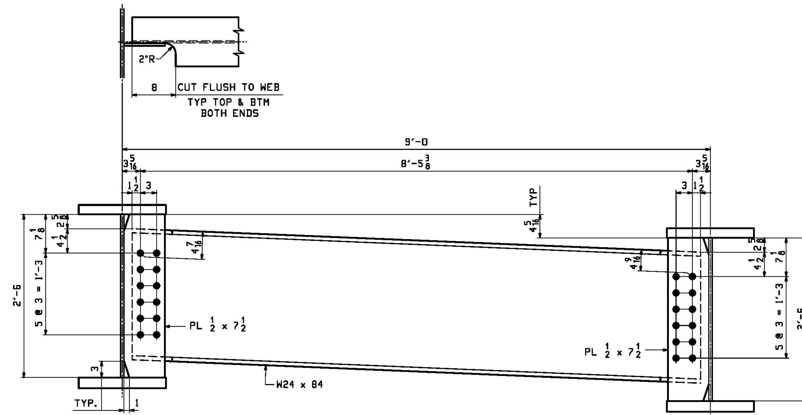
TYPICAL DIAPHRAGM LOOKING BACKSTATION TYPICAL
