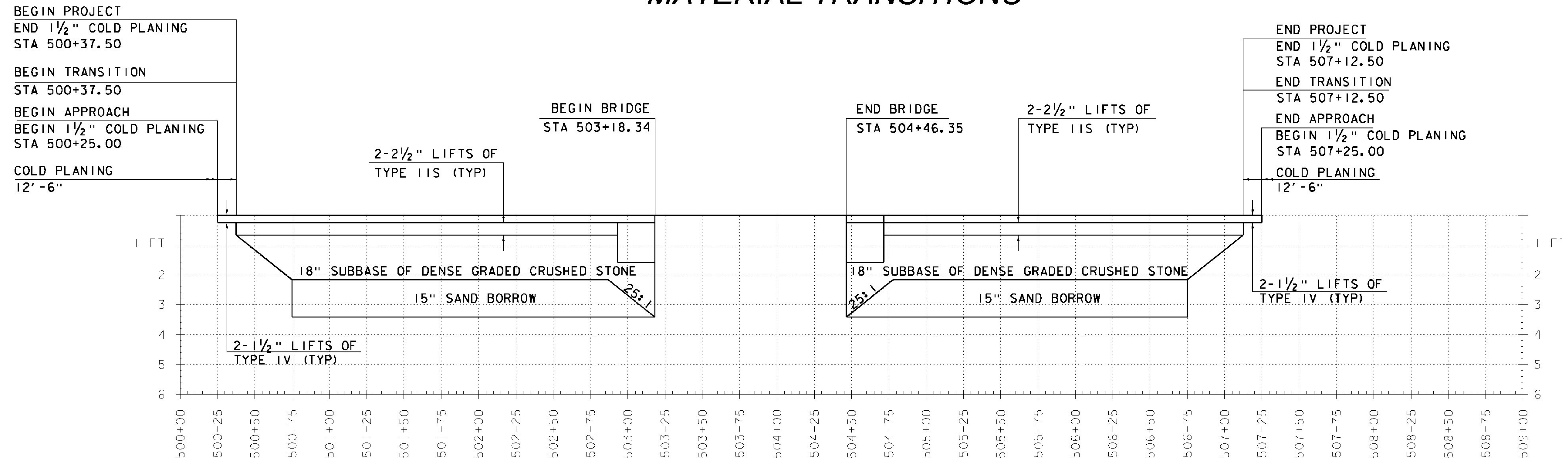
BANKING DIAGRAM & MATERIAL TRANSITION SHEET
