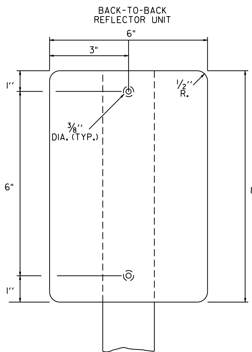
TYPE II (6"X8")
