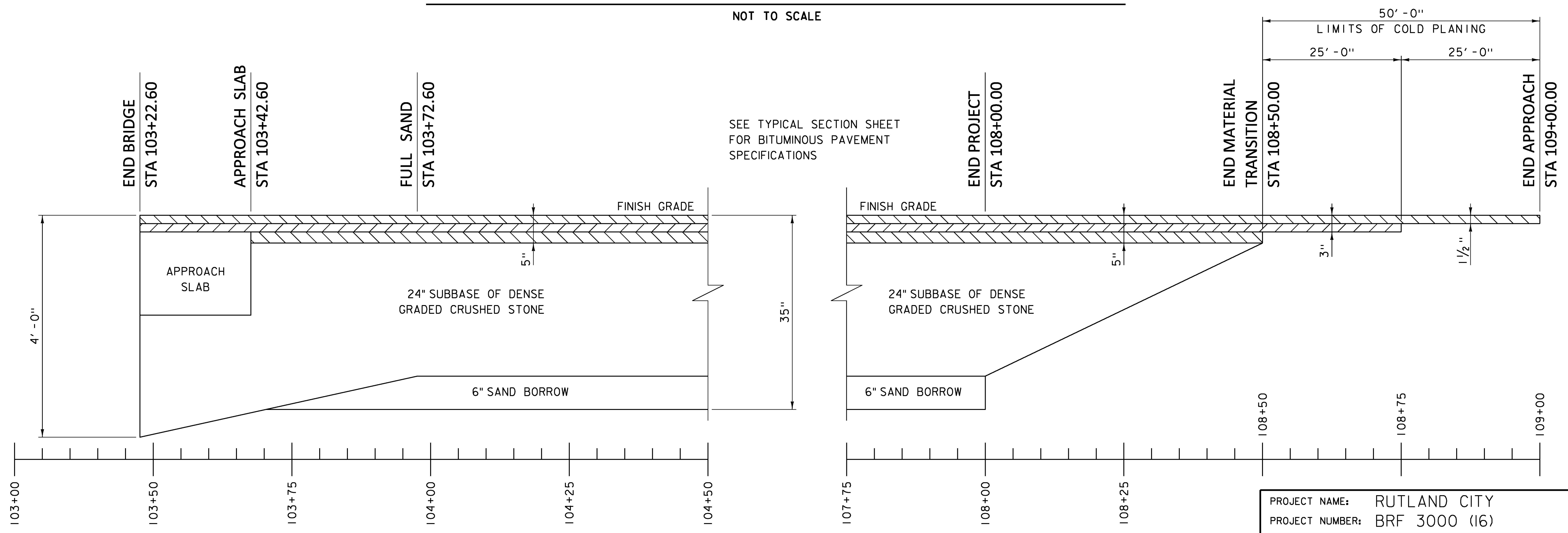
TH 8 (RIVER STREET) MATERIAL TRANSITION DETAIL NOT TO SCALE
