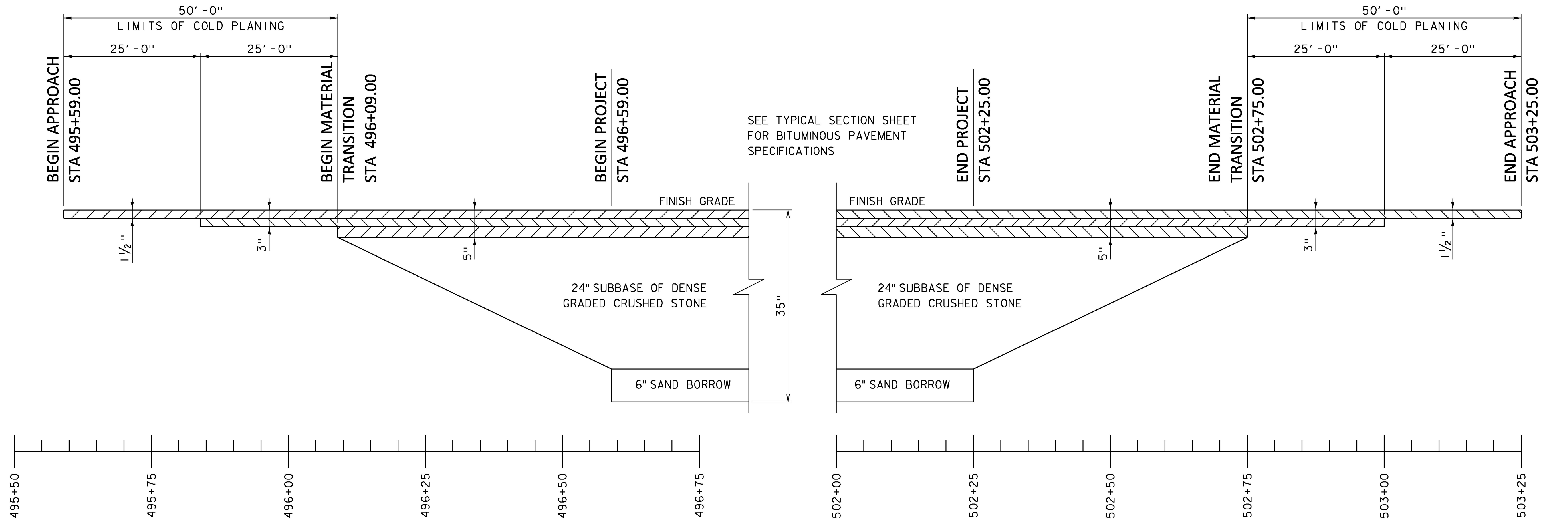
TH 10 (DORR DRIVE) MATERIAL TRANSITION DETAIL NOT TO SCALE
