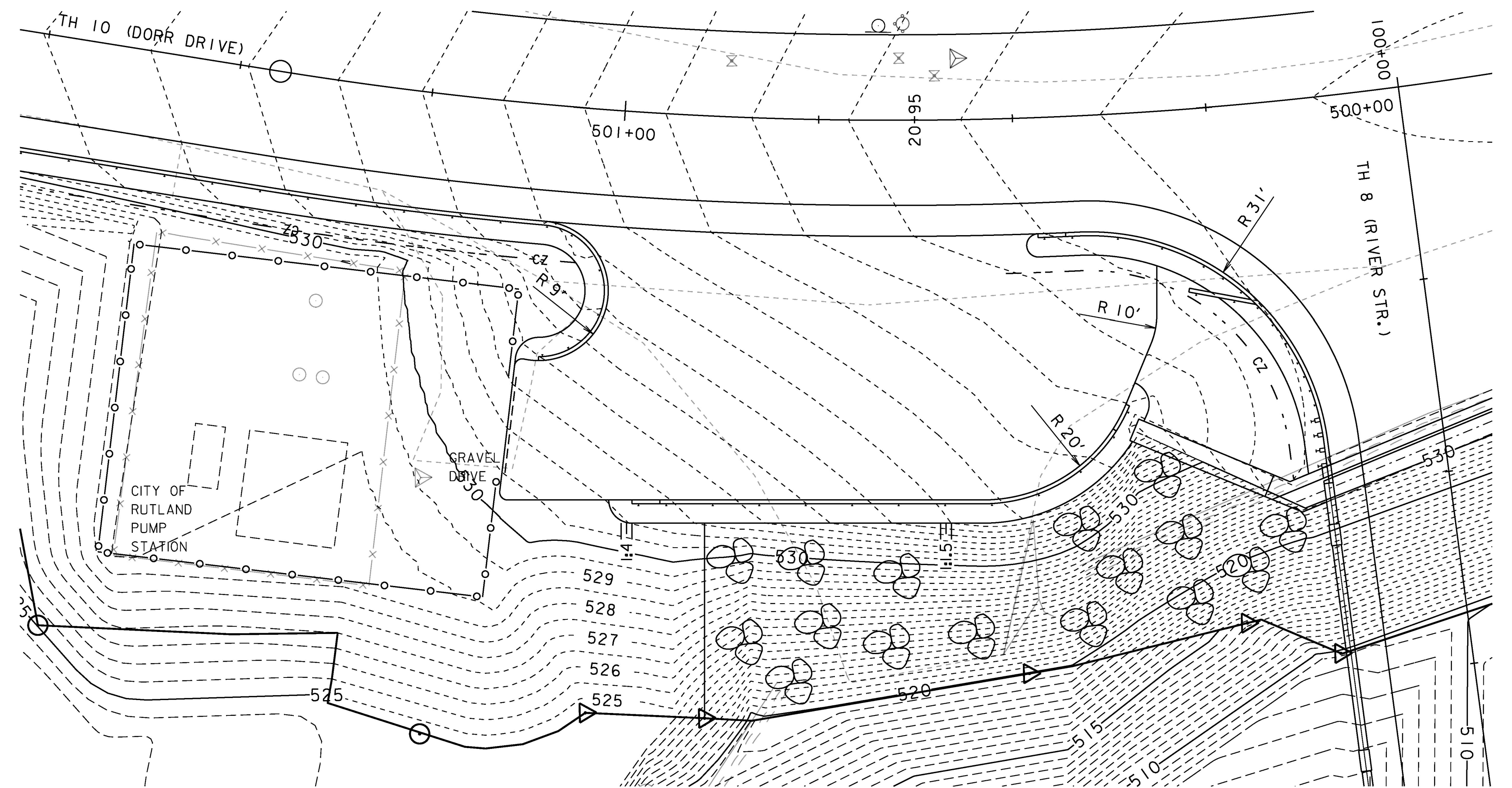
PUMP HOUSE UTILITY DRIVE PLAN SCALE 1" = 10'
