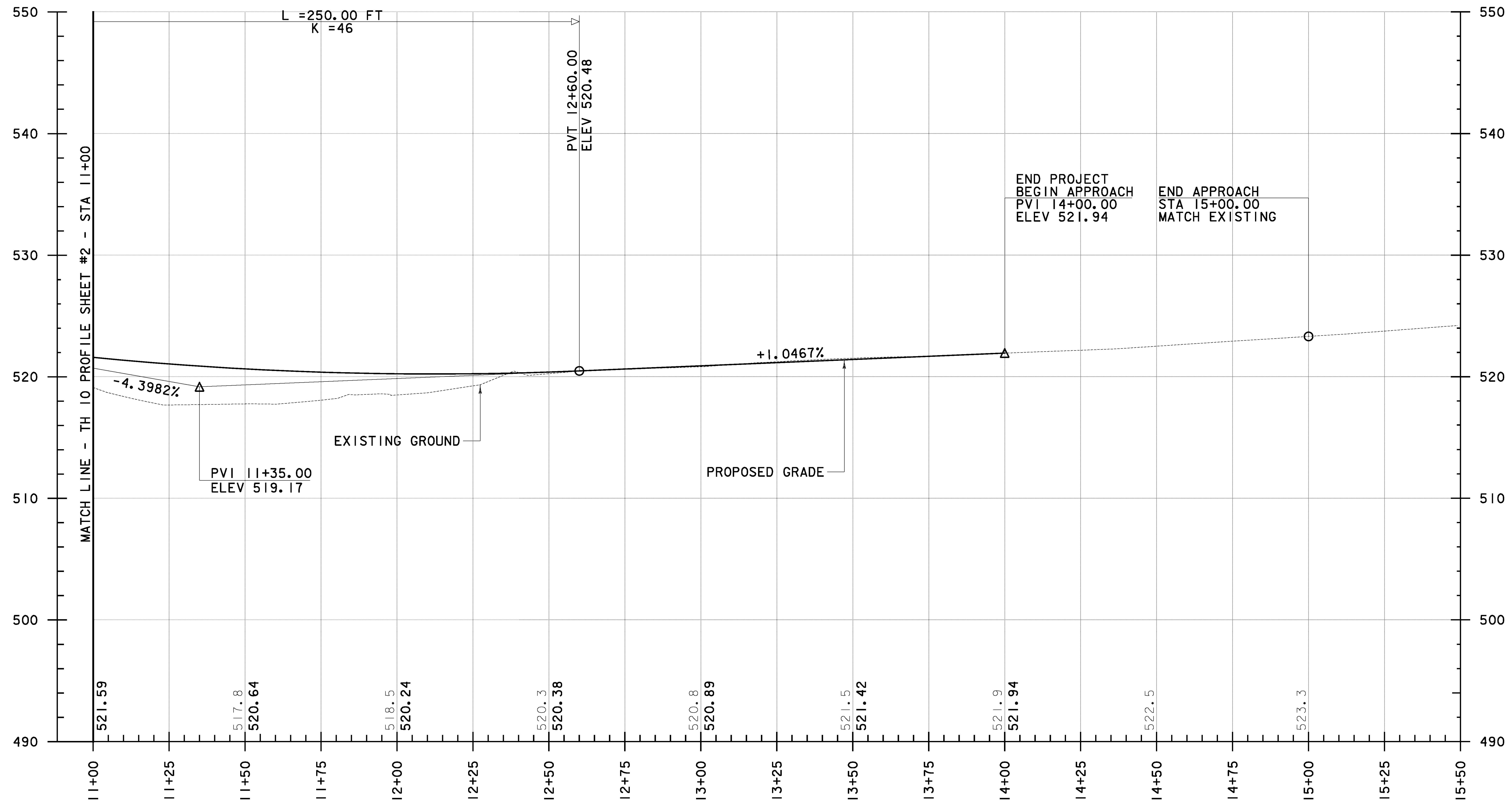
PROFILE - TH 10 SCALE IN FEET: 1" = 20' HORIZONTAL 1" = 5' VERTICAL
