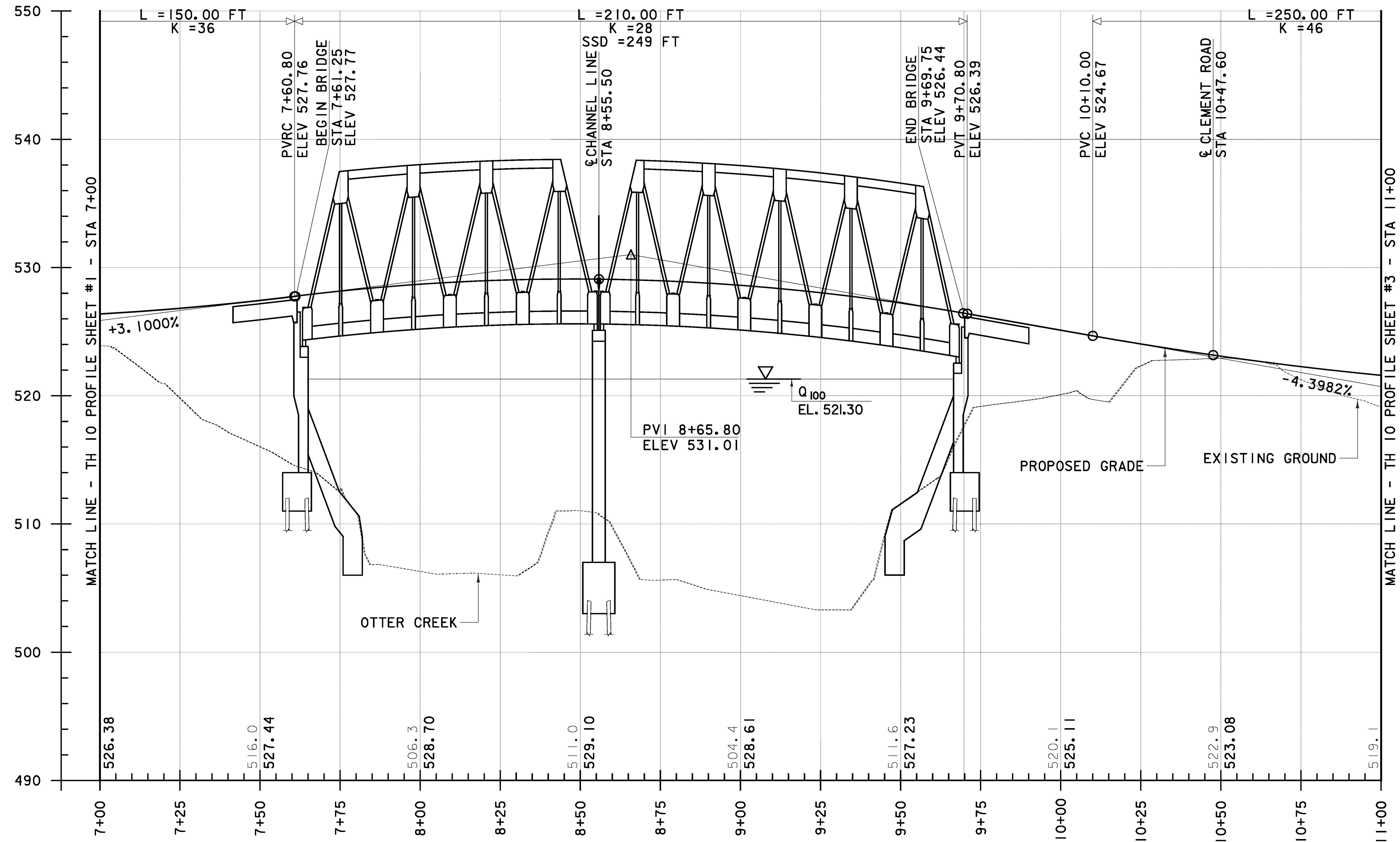
PROFILE TH 10 SCALE IN FEET: 1" = 20' HORIZONTAL 1" = 5' VERTICAL
