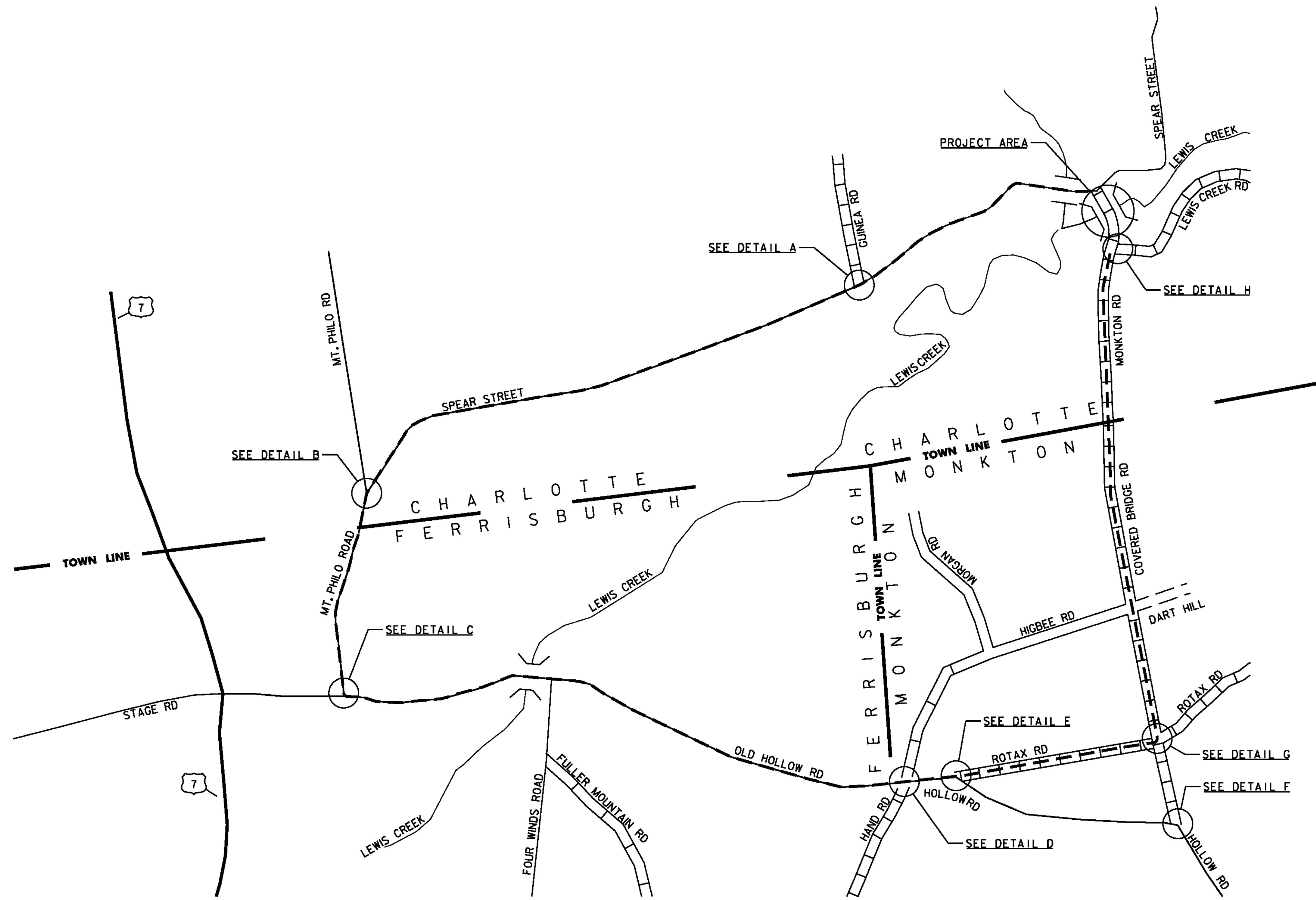
TRAFFIC CONTROL PLAN SCALE 1" = 800' 800 0 800
