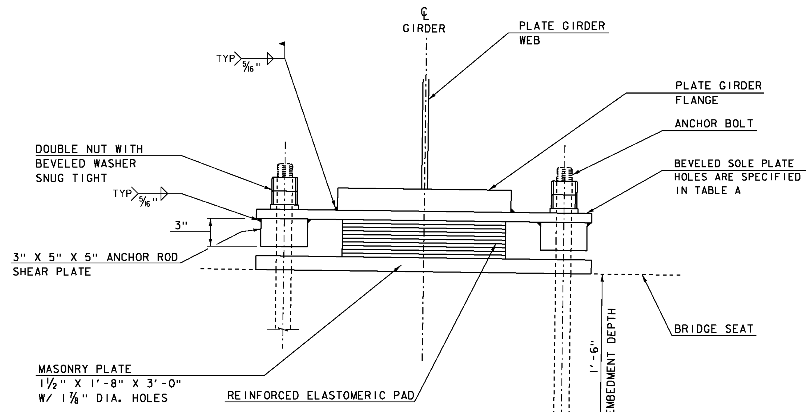
END ELEVATION SECTION B-B
