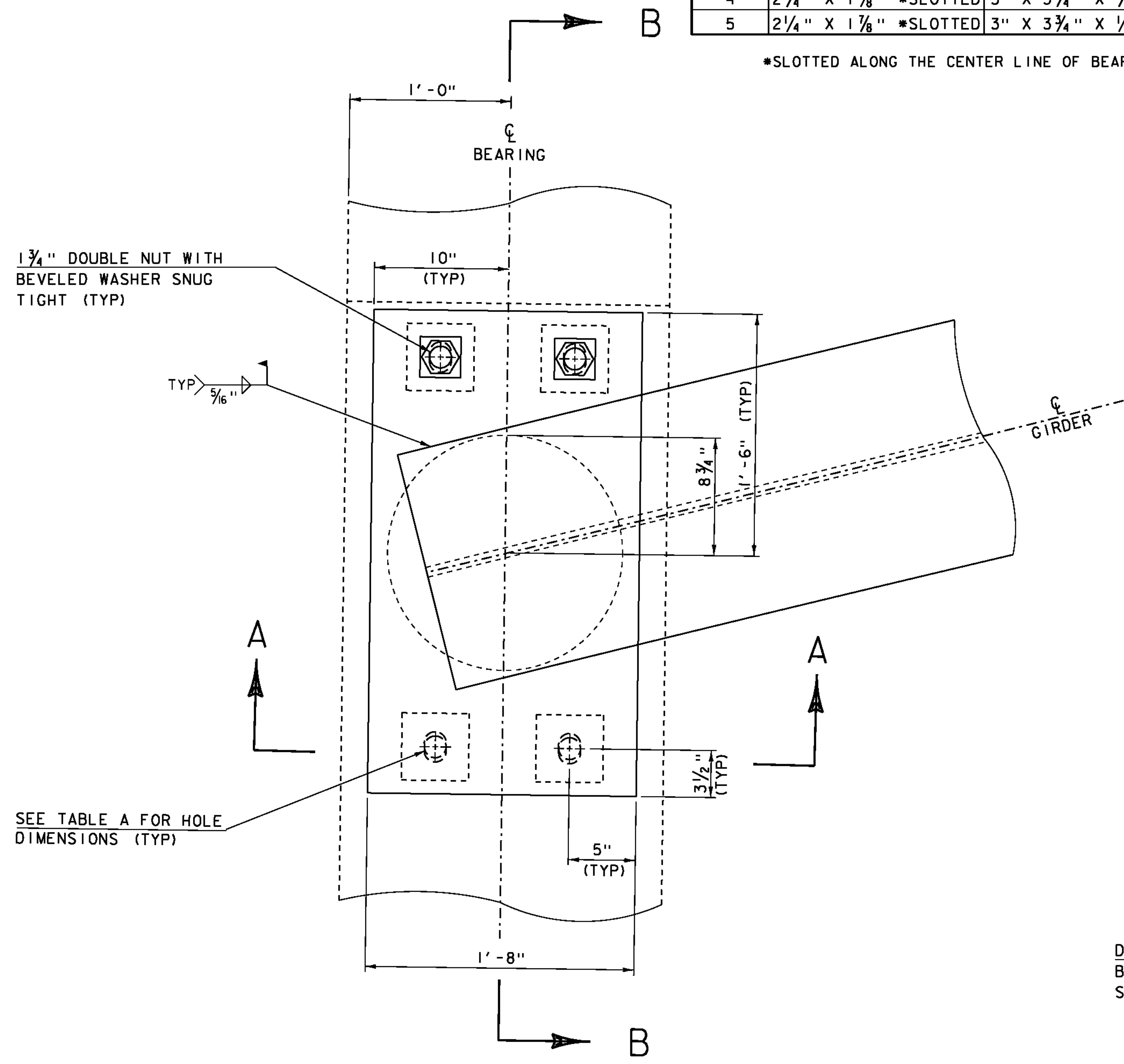
PLAN VIEW
