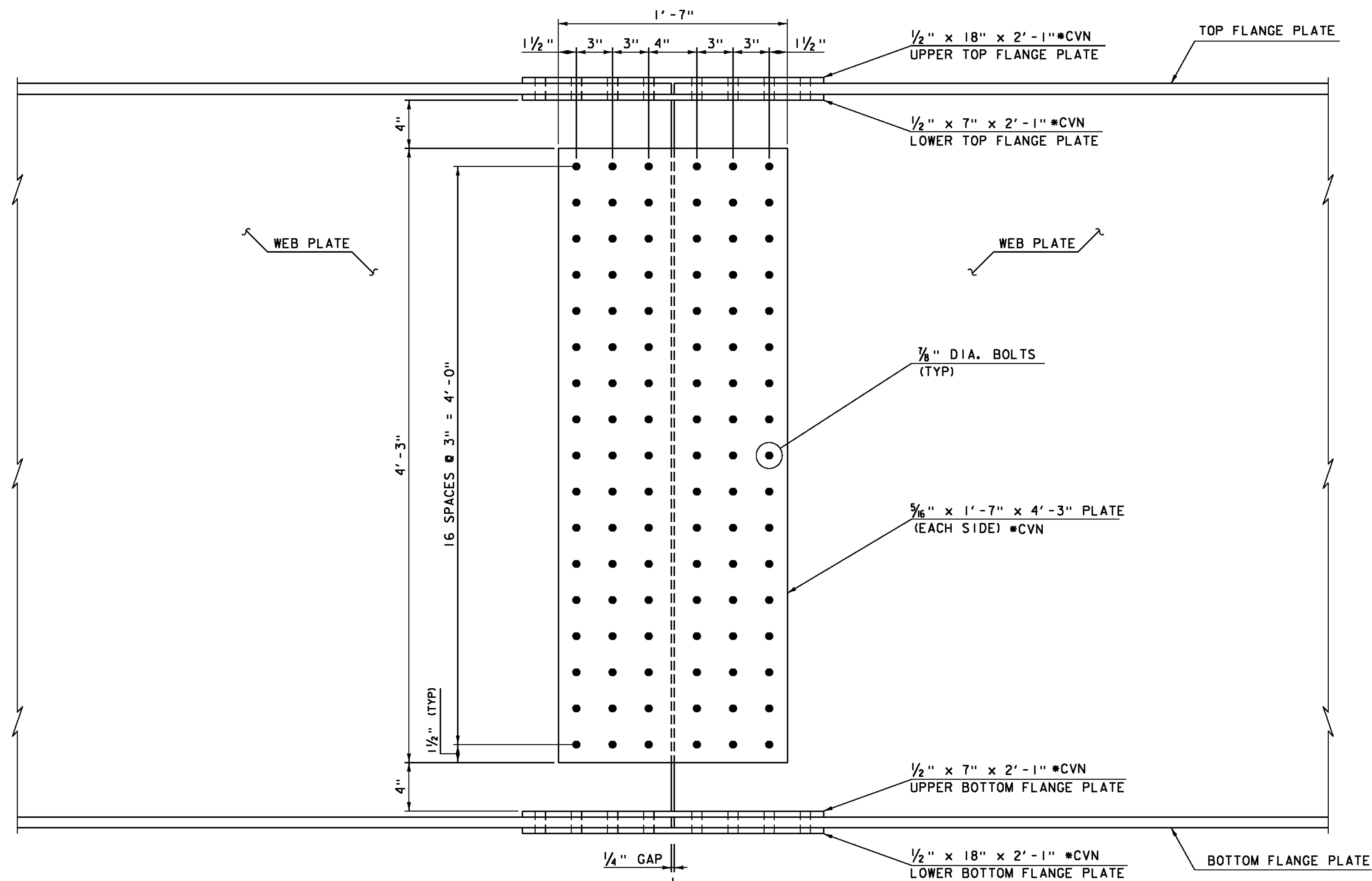
SPLICE ELEVATION GIRDERS 3, 4 & 5 SCALE 1" = 1'-0"
