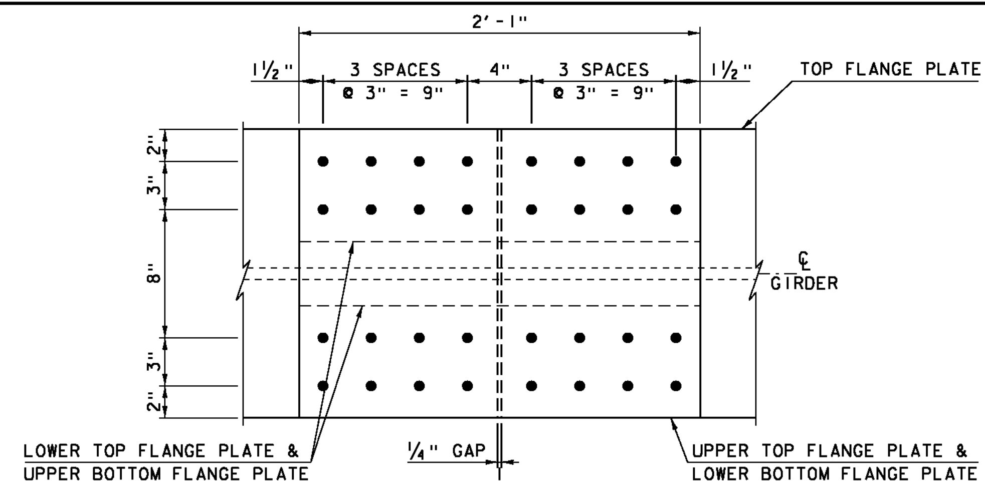
TOP & BOTTOM FLANGE PLAN GIRDERS 3, 4 & 5 SCALE 1" = 1'-0"
