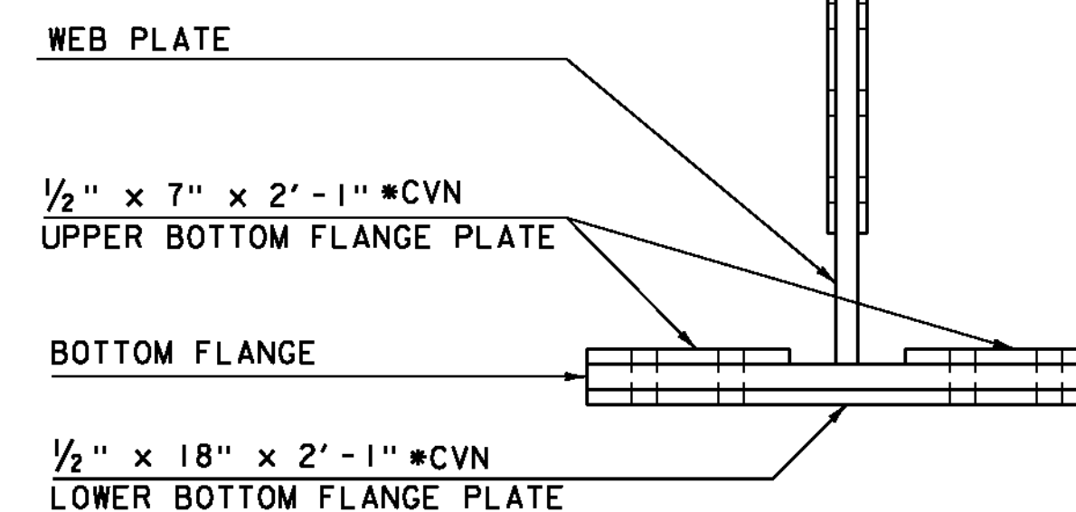
SPLICE SECTION GIRDERS 3, 4 & 5 SCALE 1" = 1'-0"
